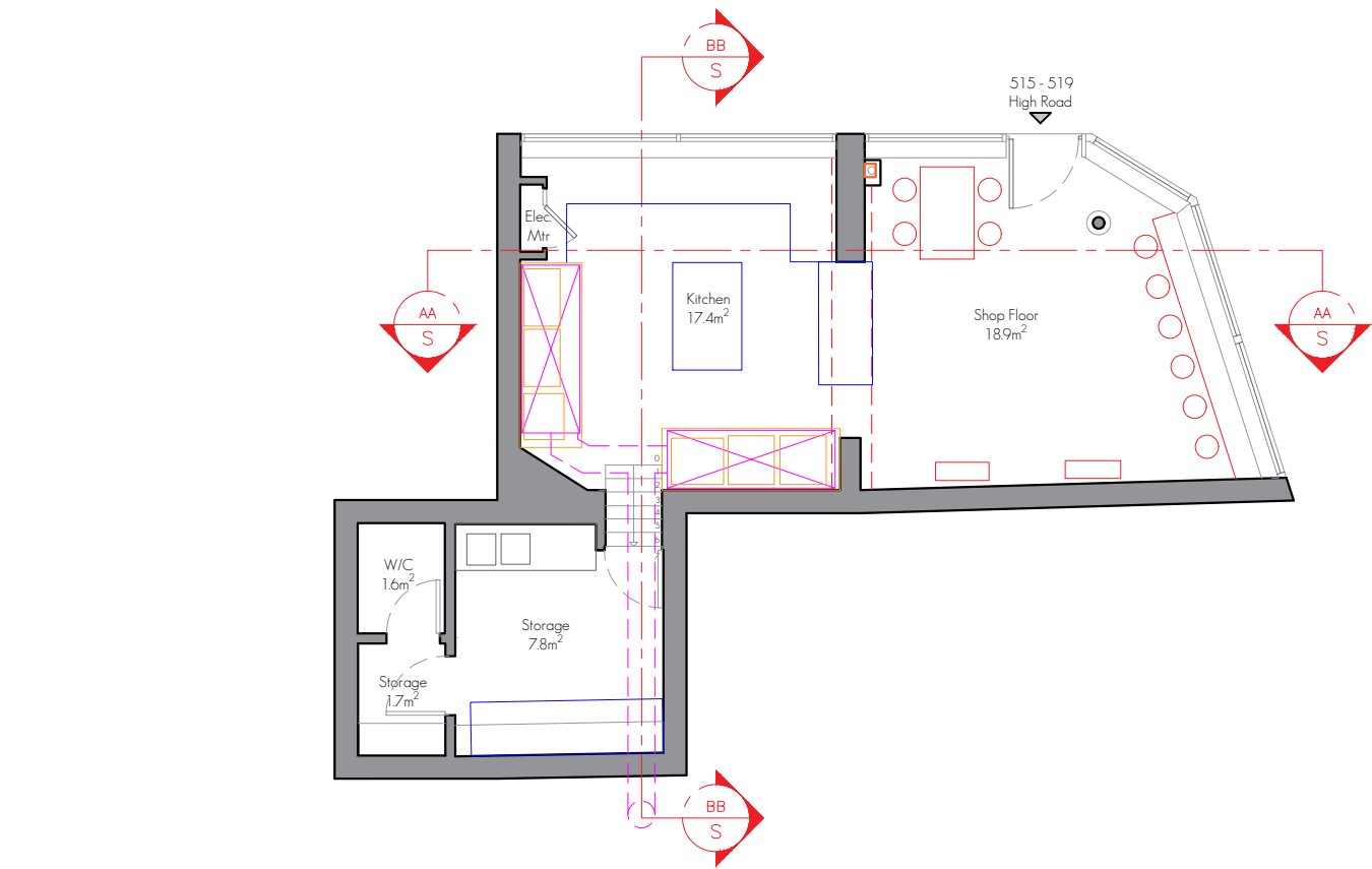
PROPOSED GROUND FLOOR PLAN Gross Internal Area (GIA): 52.9m 2
