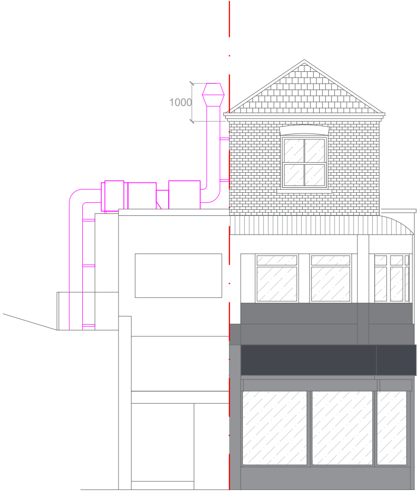
PROPOSED SIDE (SOUTH) ELEVATION
