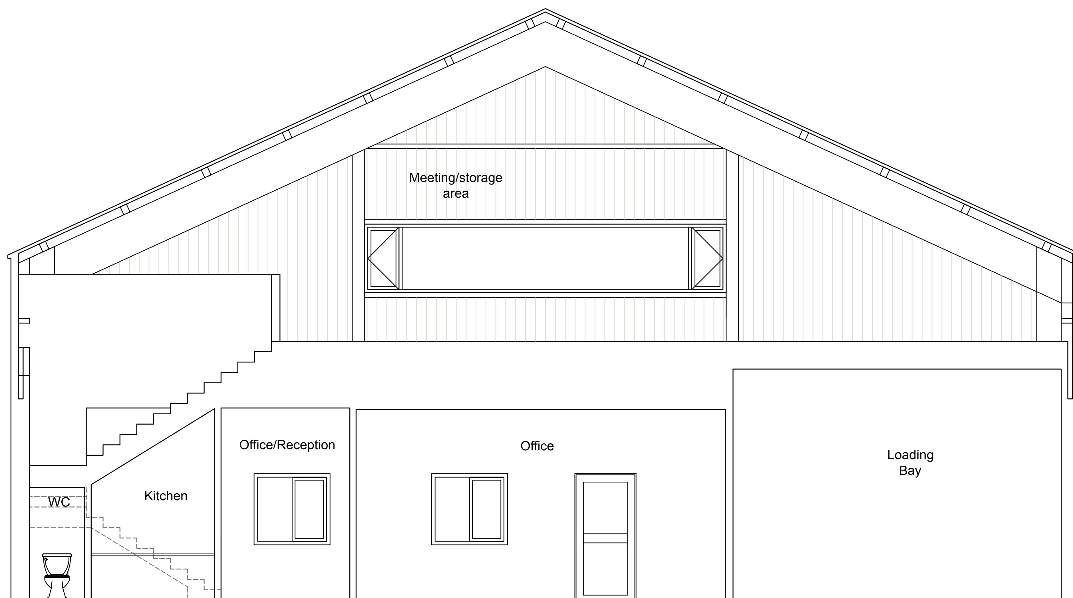
Proposed Section AA
