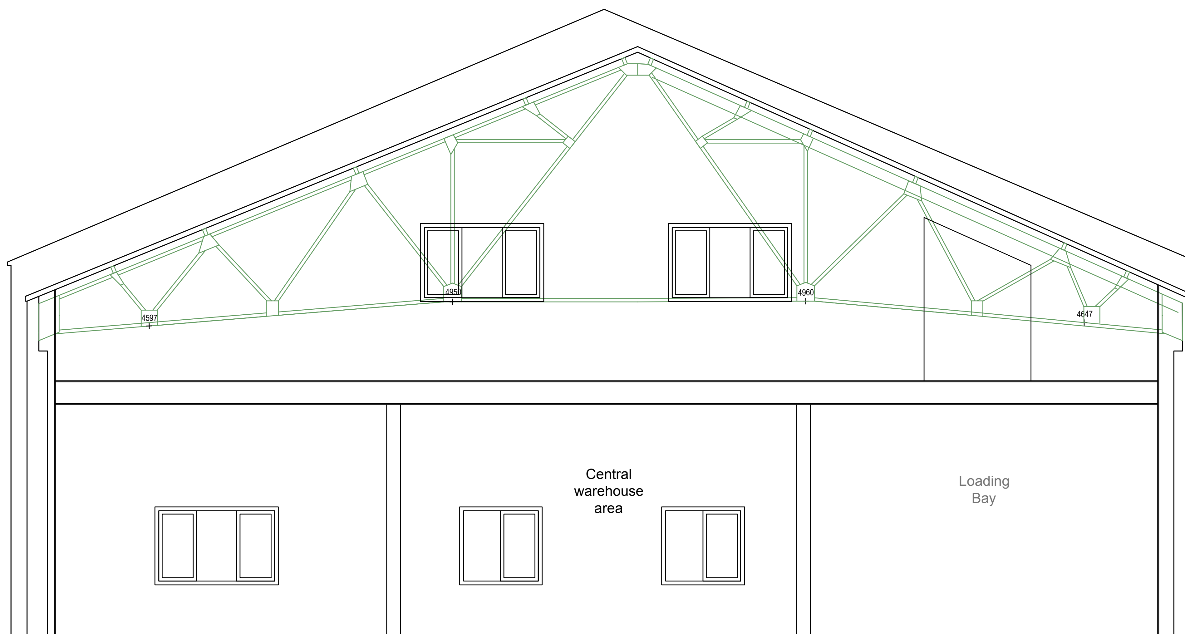
Proposed Section BB
