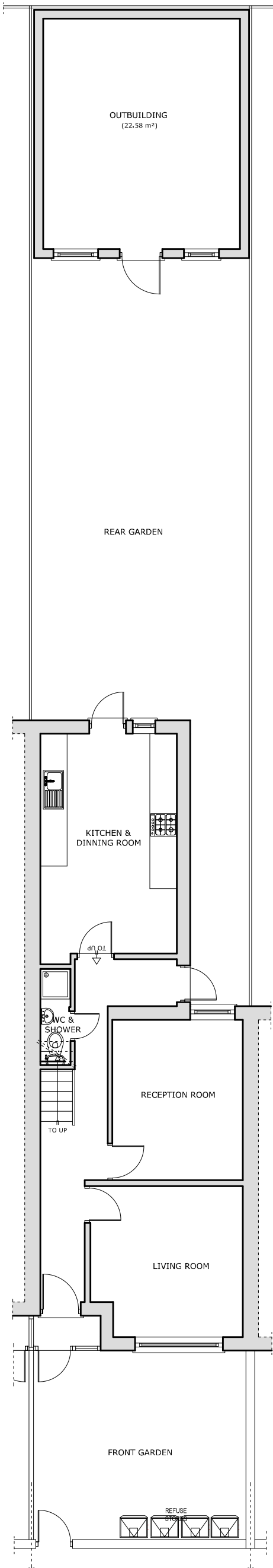
EXISTING GROUND FLOOR PLAN
