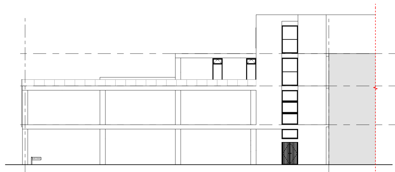
Side elevation as existing
