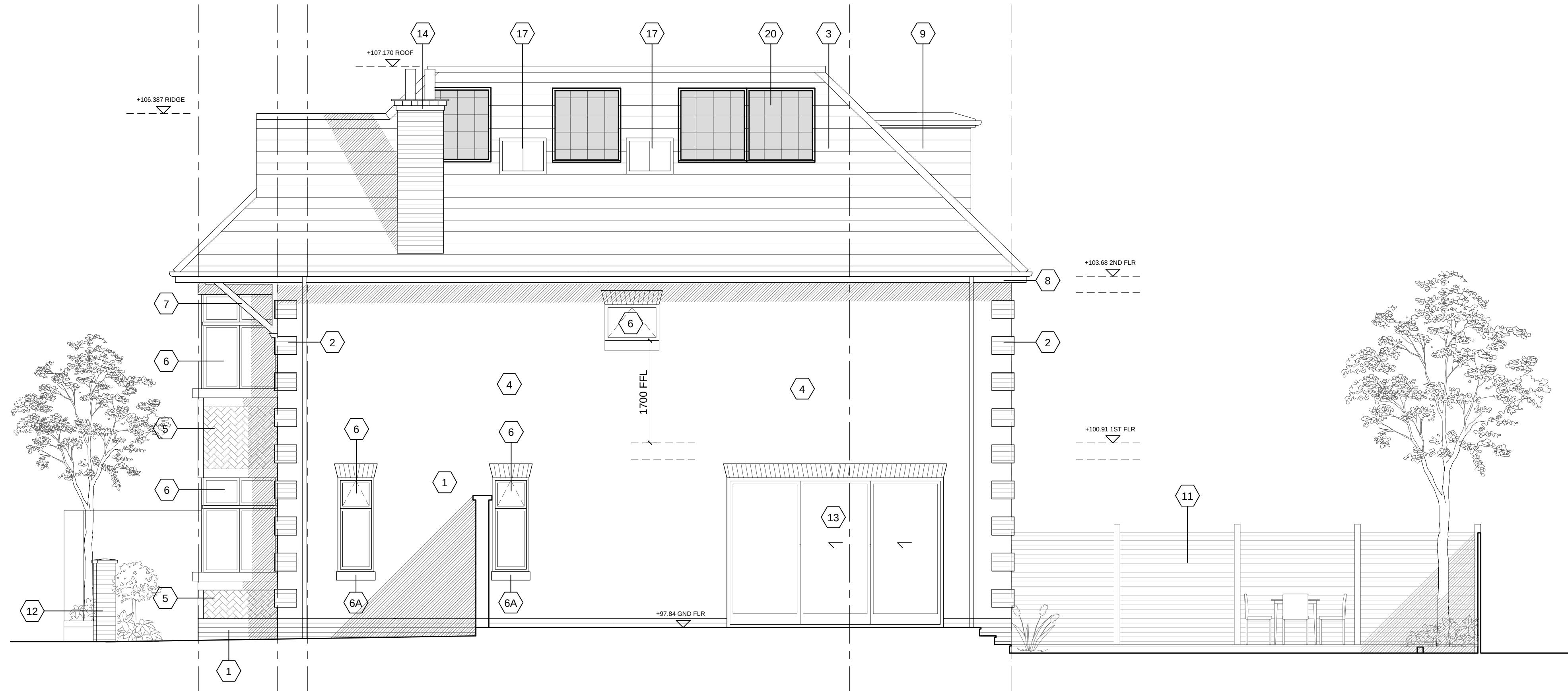
PROPOSED SIDE ELEVATION C
