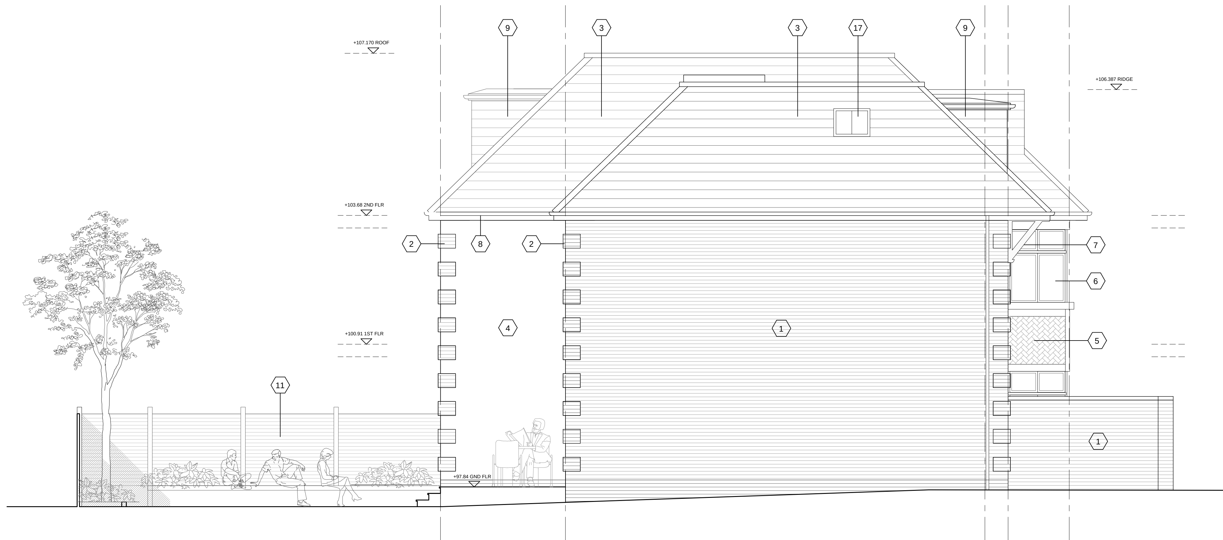
PROPOSED SIDE ELEVATION C
