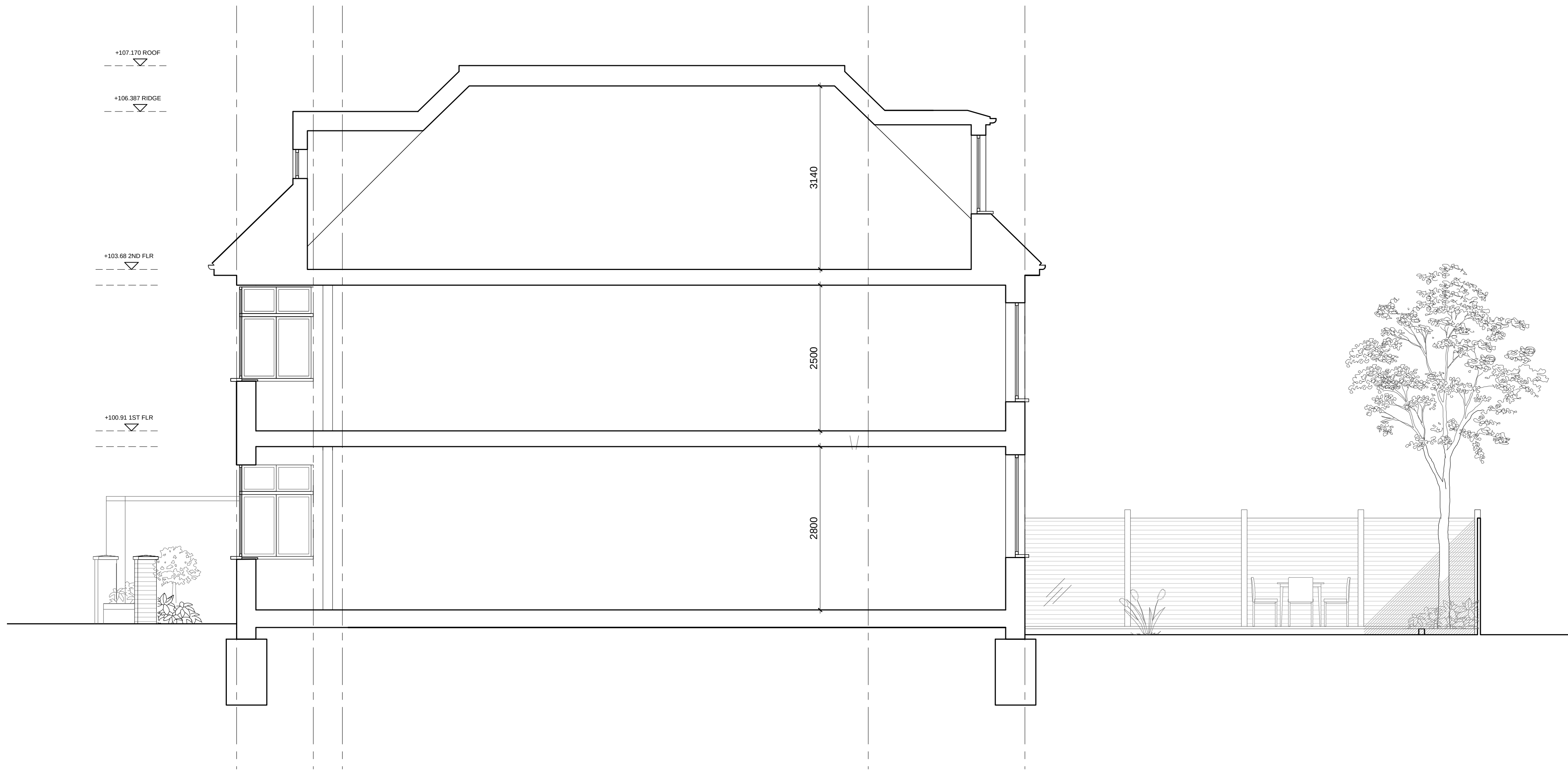
PROPOSED SIDE ELEVATION C
