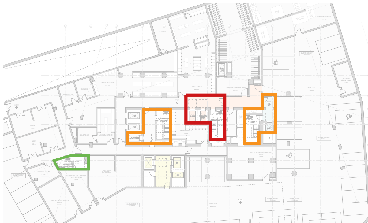
FIGURE 325. Basement General Arrangement Plan
