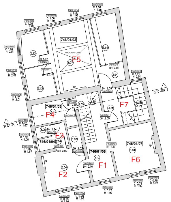
Dispensary First Floor As Existing
