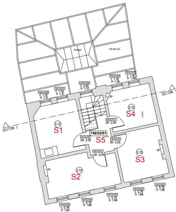
Dispensary Second Floor As Existing
