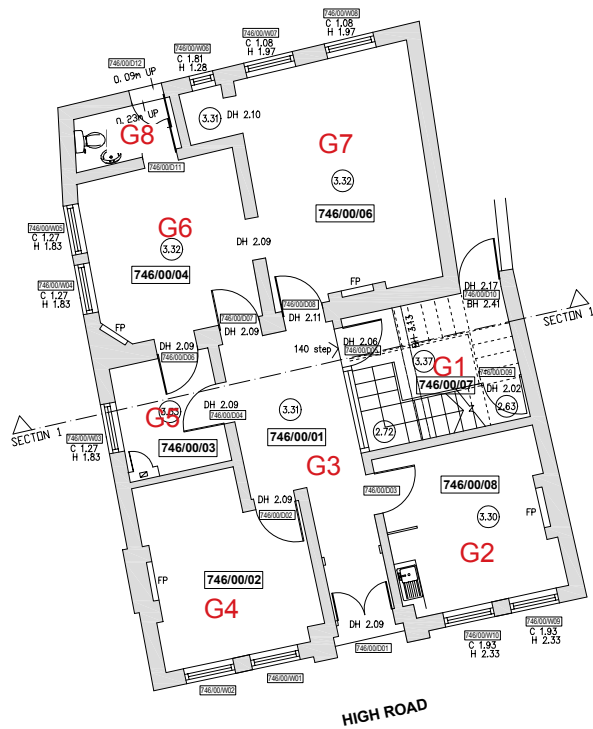
Dispensary Ground Floor As Existing
