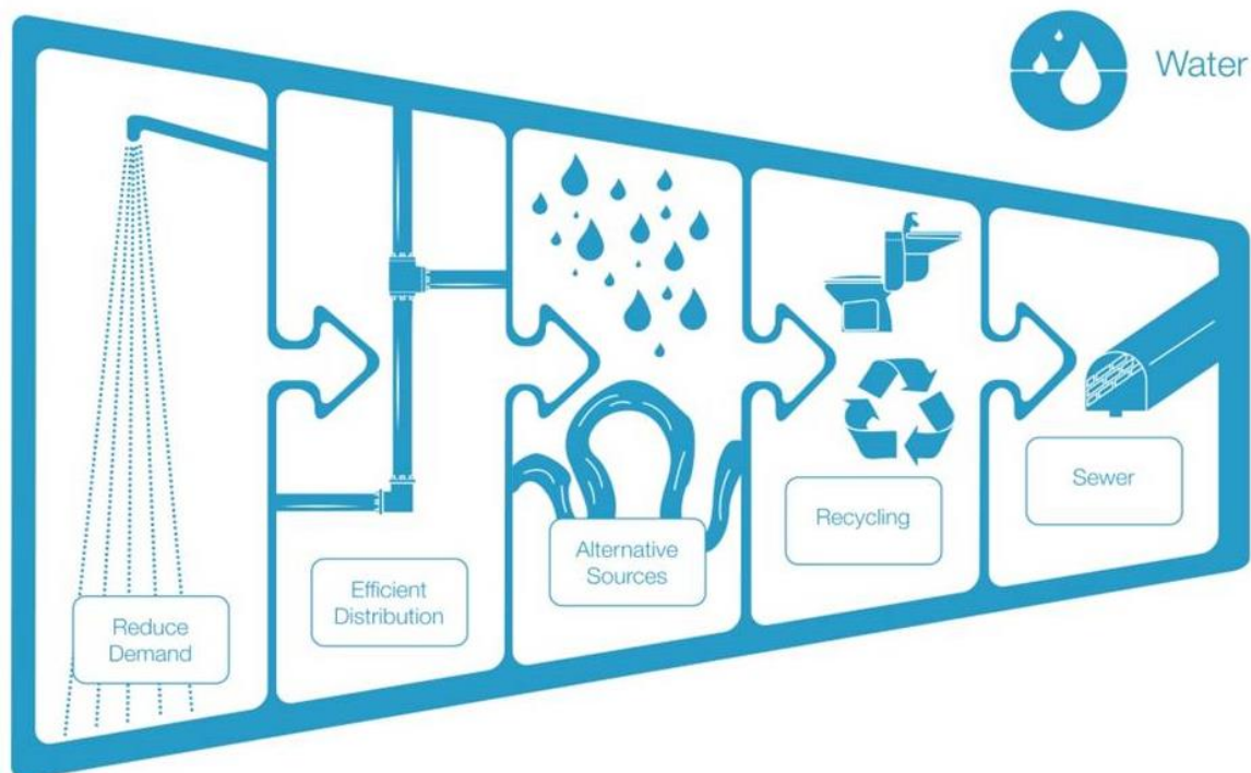
Figure 4-1 Water hierarchy
