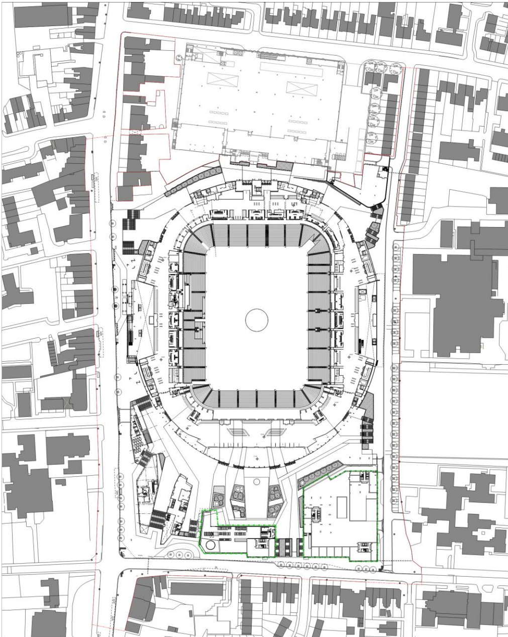
Figure 2-2 Northumberland Development Masterplan
