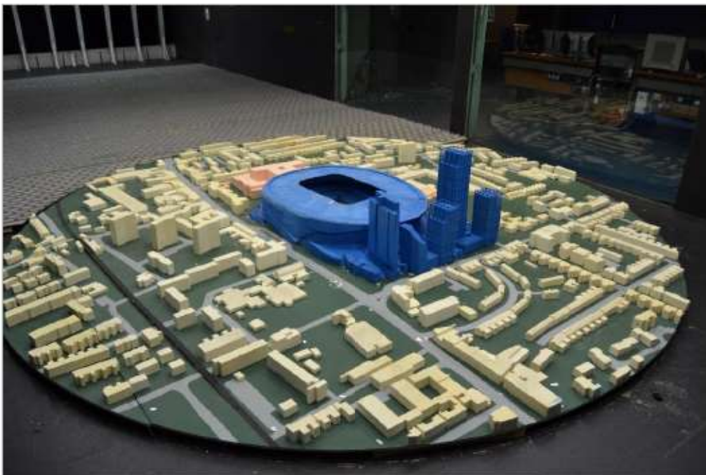
Figure B.8: Wind tunnel set-up, viewed from downstream
