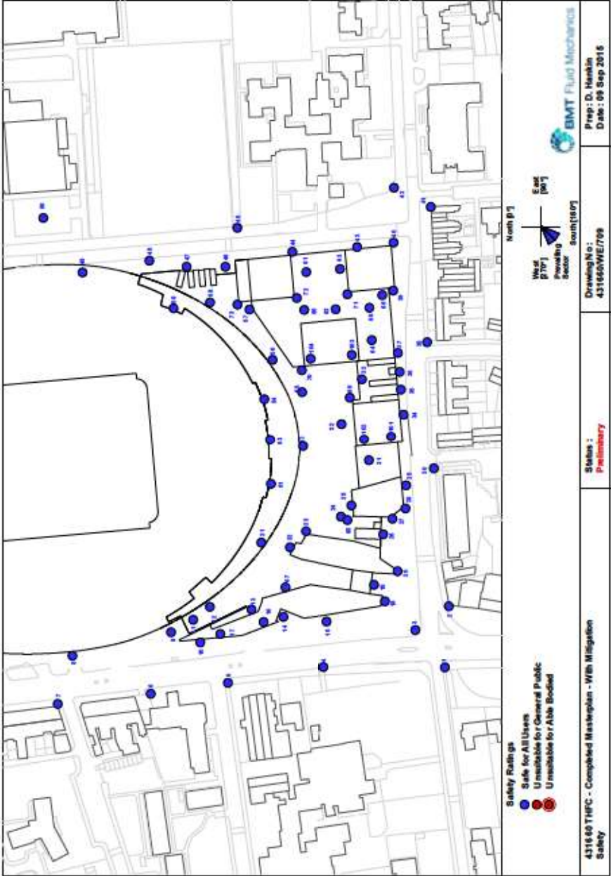
Figure D.11: Annual safety ratings, the completed masterplan, southern podium area, with soft landscaping and wind mitigation
