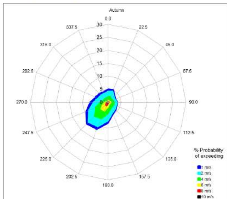
Figure A.5d: Directional Windspeed Probability Distribution at Site: Autumn (at 50m height)
