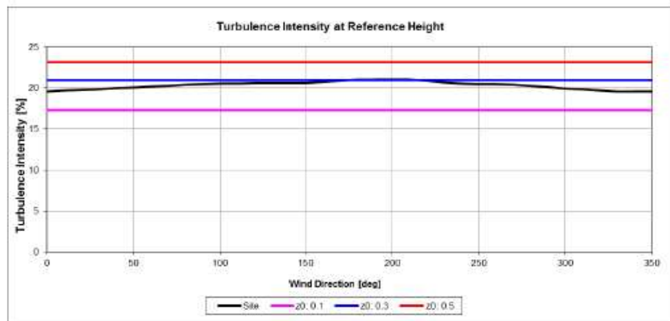
Figure A.1: Variation of turbulence intensity with wind direction at 50m height, including reference turbulence levels
