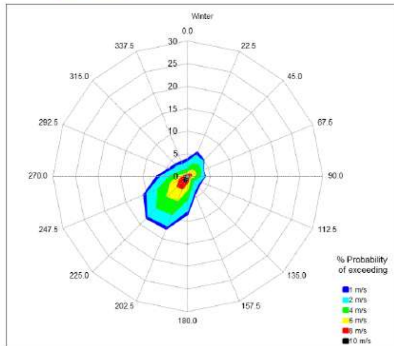
Figure A.5e: Directional Windspeed Probability Distribution at Site: Winter (at 50m height)
