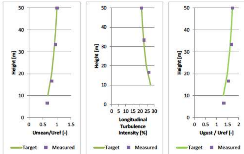
Figure A.4: Mean wind speed ( U_{\text{mean}}/U_{\text{mean(ref)}} ), longitudinal turbulence intensity profiles ( I_u ) and gust wind speed ( U_{\text{gust}}/U_{\text{mean(ref)}} ) modelled in the study
