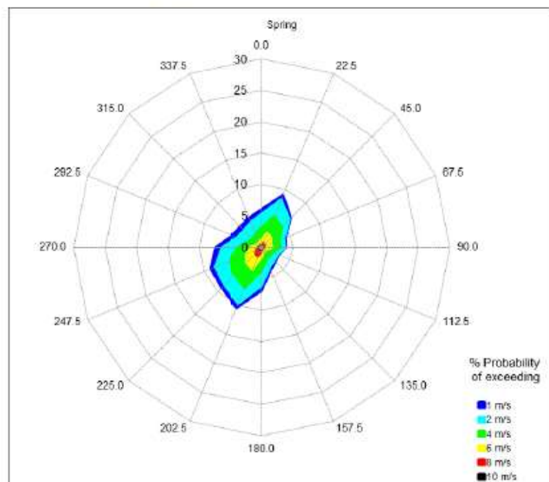
Figure A.5b: Directional Windspeed Probability Distribution at Site: Spring (at 50m height)
