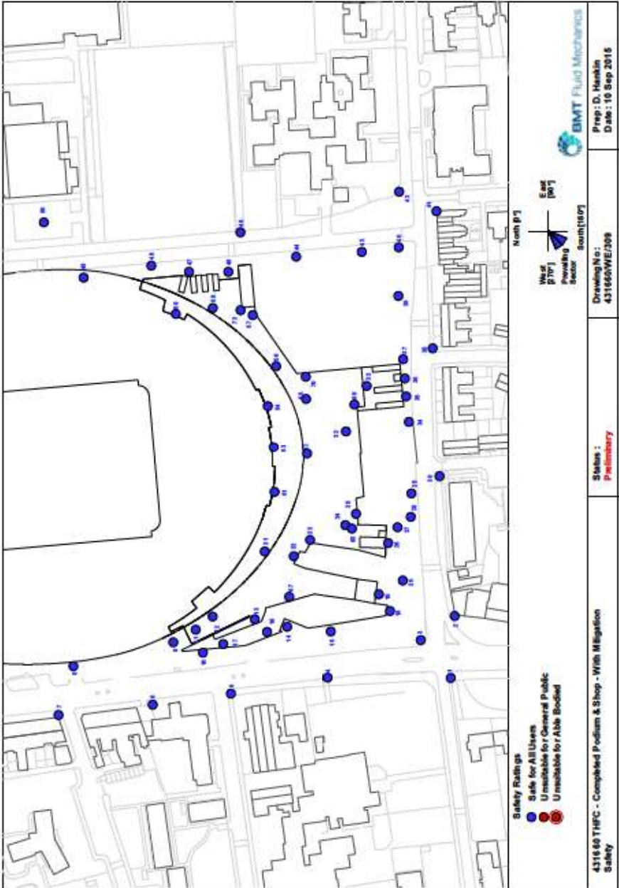
Figure D.1e: Annual safety ratings, the completed podium, southern podium area, with soft landscaping and wind mitigation
