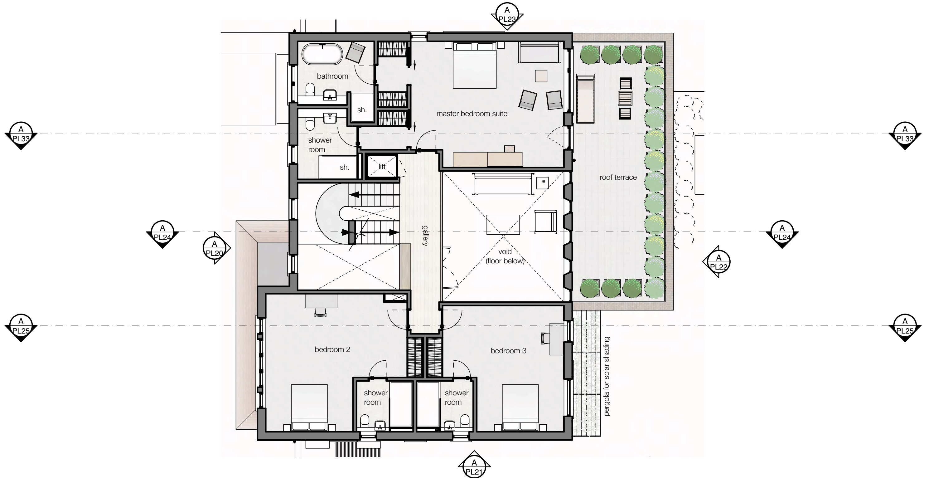
A PL16 Proposed First Floor Plan 1:100
