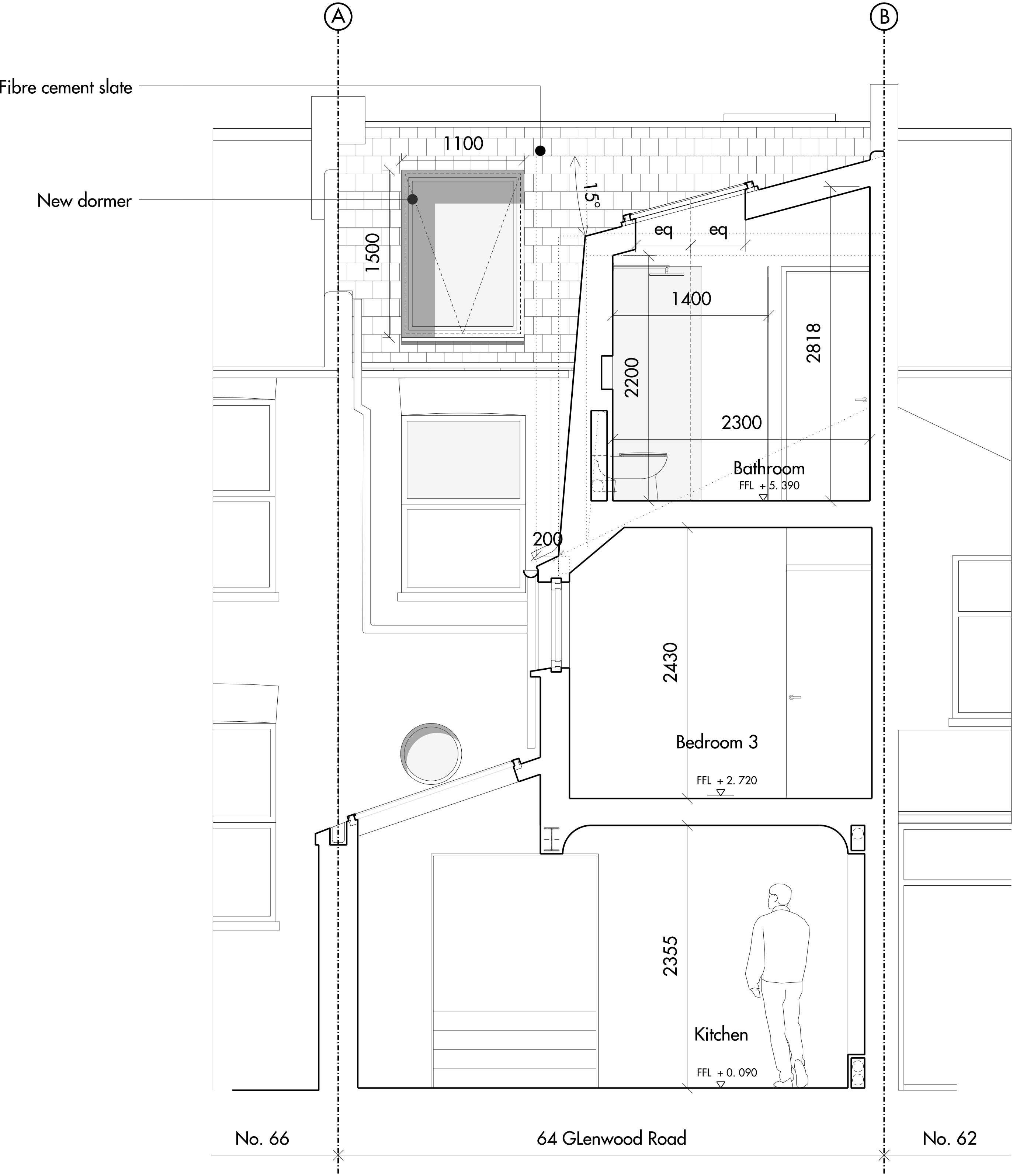
02 Proposed Section C_C 1:50 @ A3
