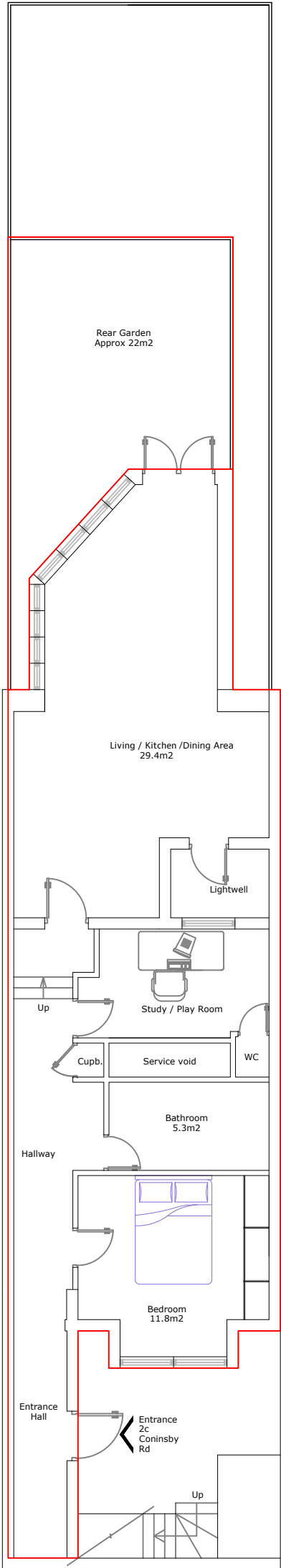
EXISTING FLOOR PLANS SCALE 1:100
