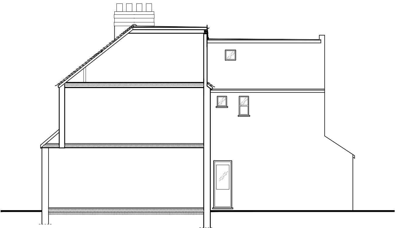
EXISTING SIDE ELEVATION & SECTION SCALE: 1/100
