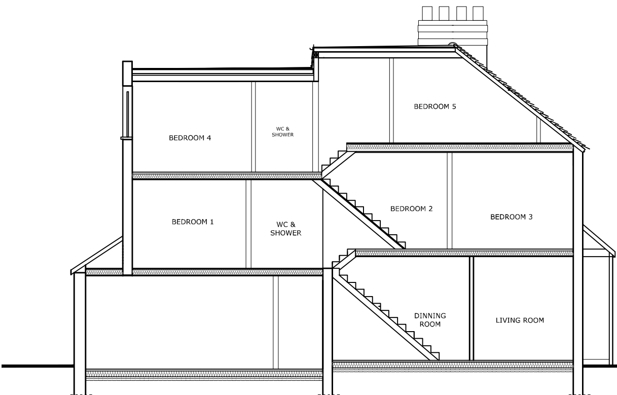
EXISTING SIDE ELEVATION & SECTION SCALE: 1/100
