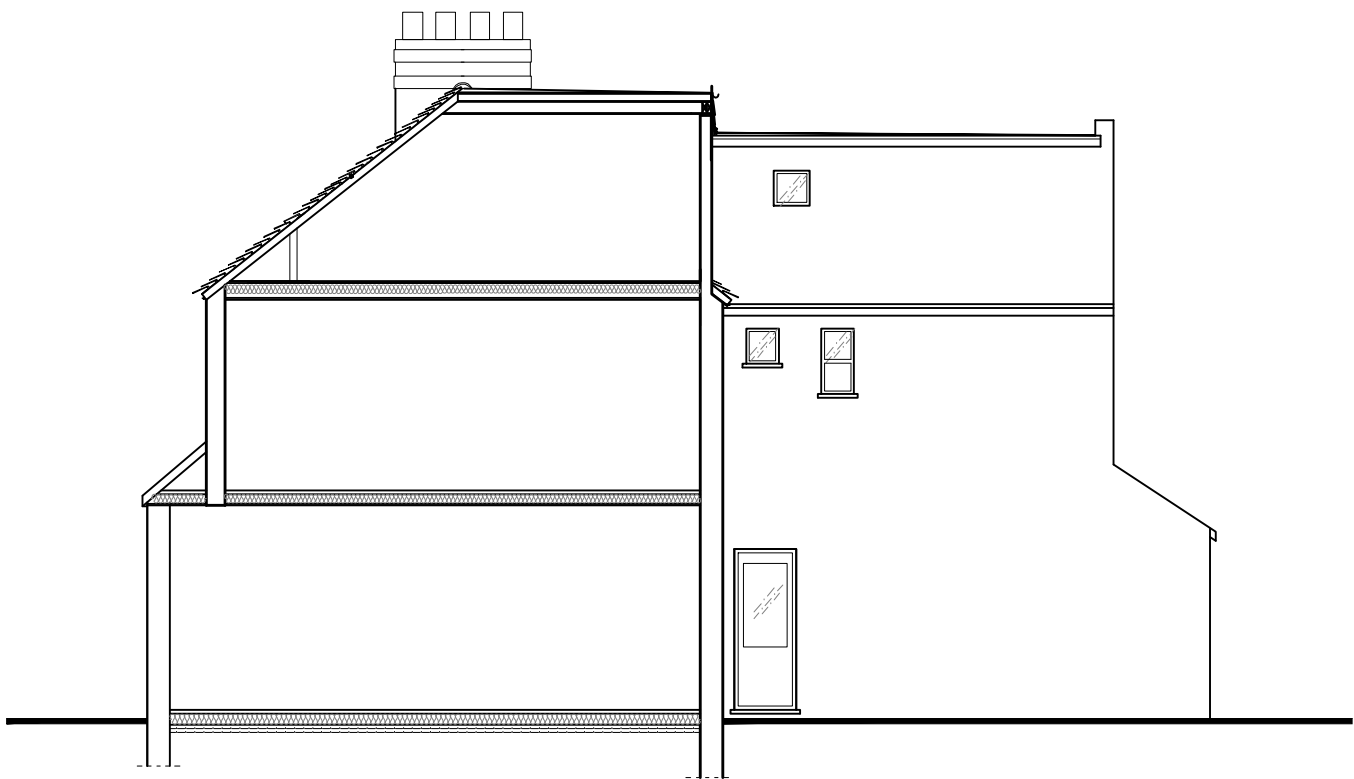
PROPOSED SIDE ELEVATION & SECTION (AS EXISTING) SCALE: 1/100
