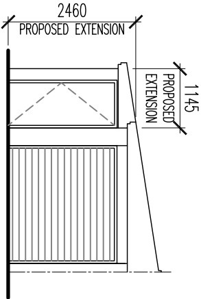
1 PROPOSED FRONT ELEVATION 1:100
