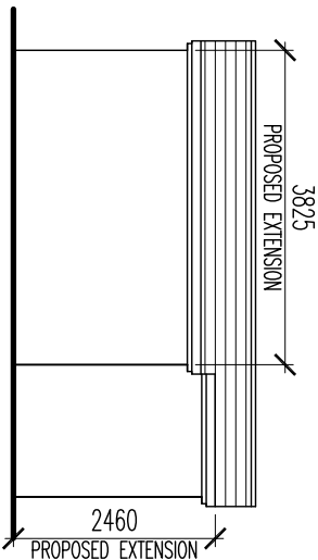
3 PROPOSED SIDE ELEVATION 1:100
