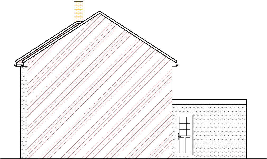
Existing Side Elevation - B
