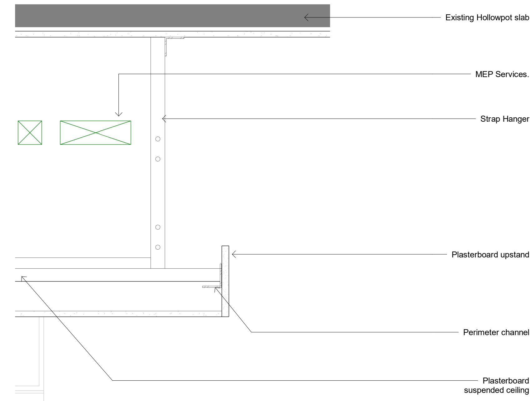
5 Ceiling Raft Detail 1:5
