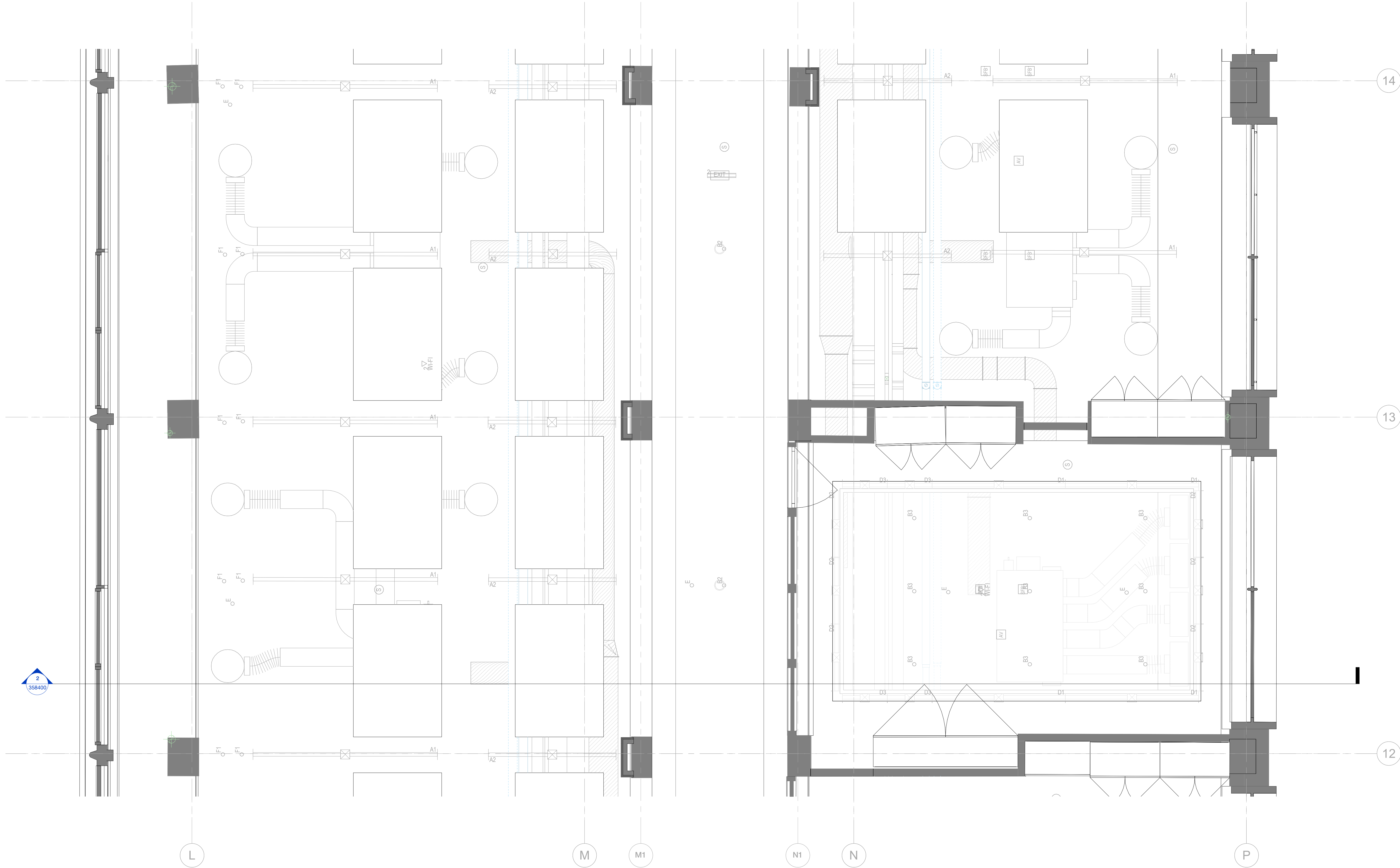
1 North Wing Typical Bay - RCP 1:25
