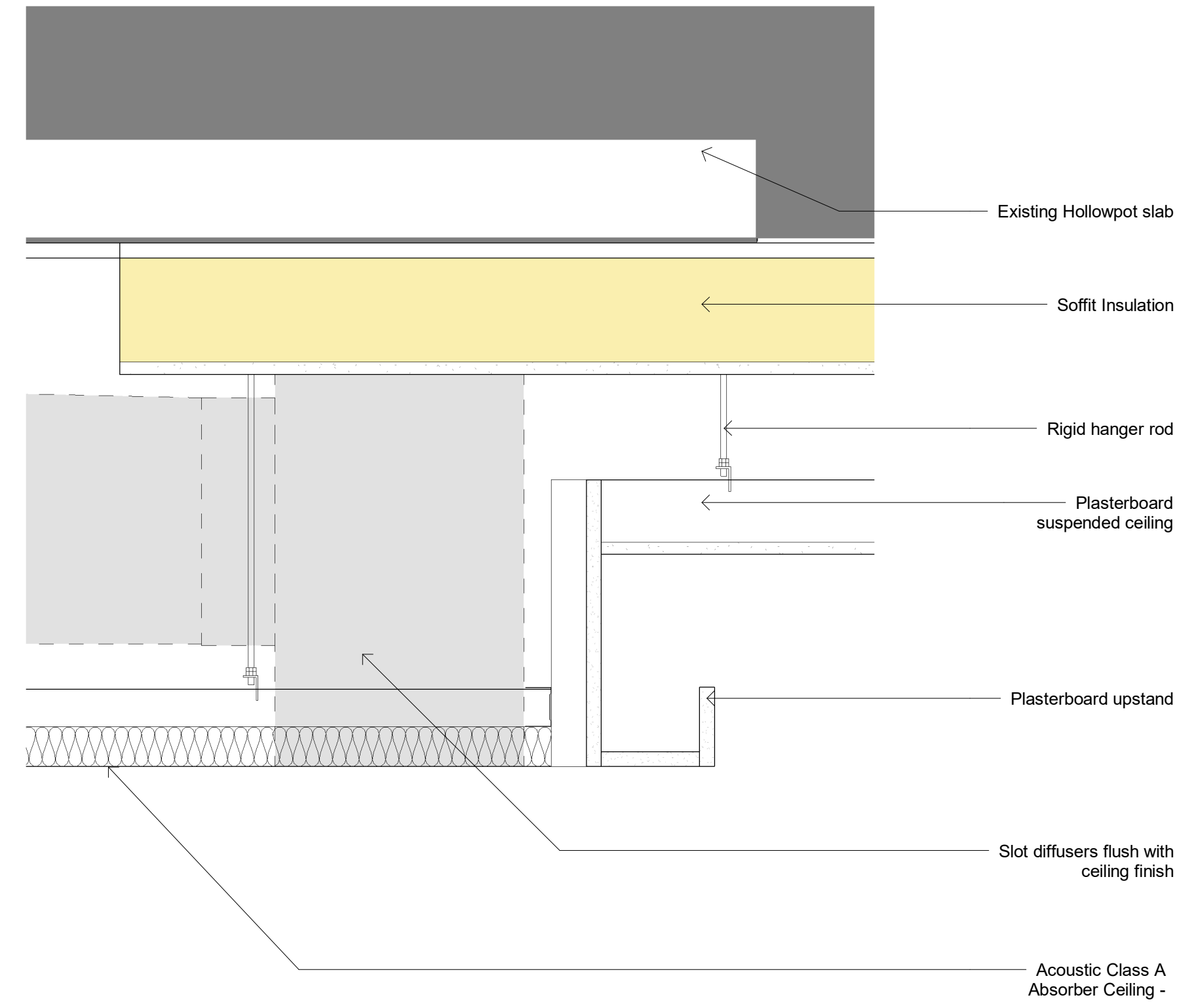
4 Cove Lighting Detail 1:5
