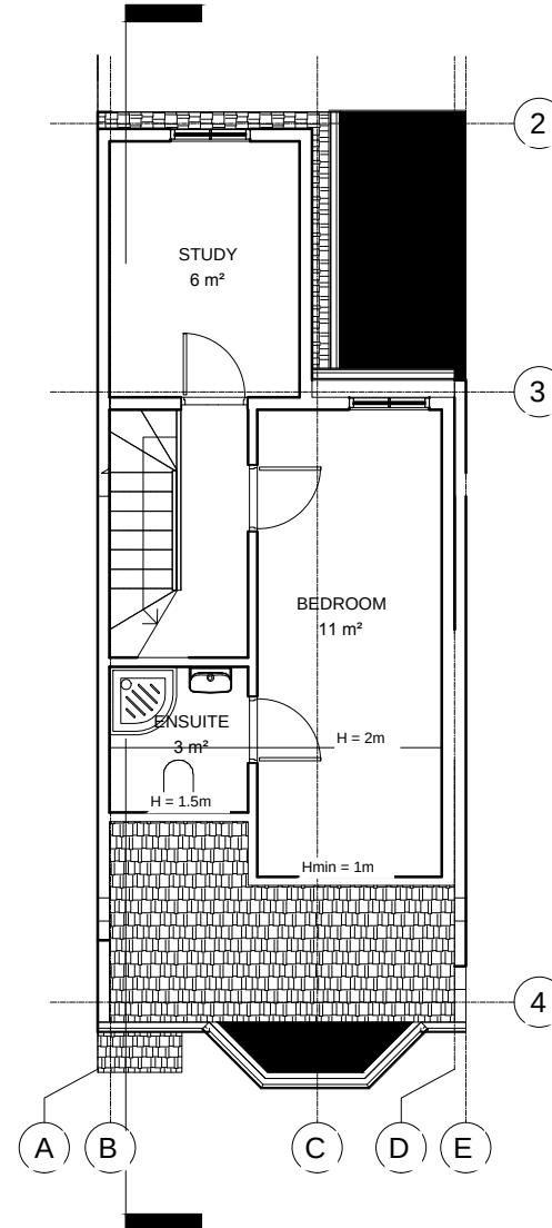
PROPOSED LOFT PLAN
