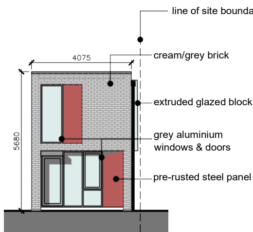
proposed front elevation 1:100 (unchanged)
