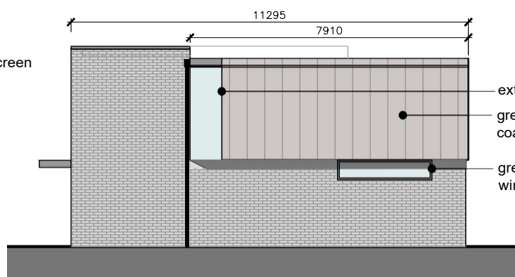
proposed side elevation 1:100 (unchanged)
