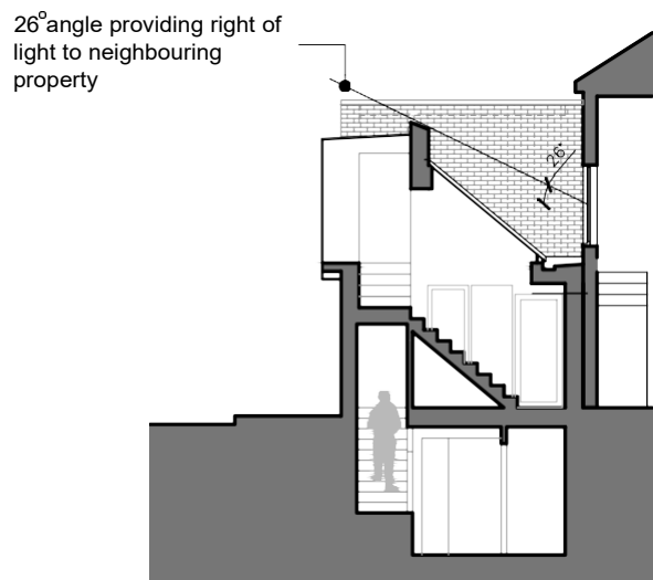
proposed section 1:100
