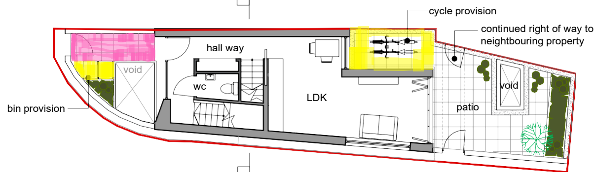
proposed ground floor plan 1:100
