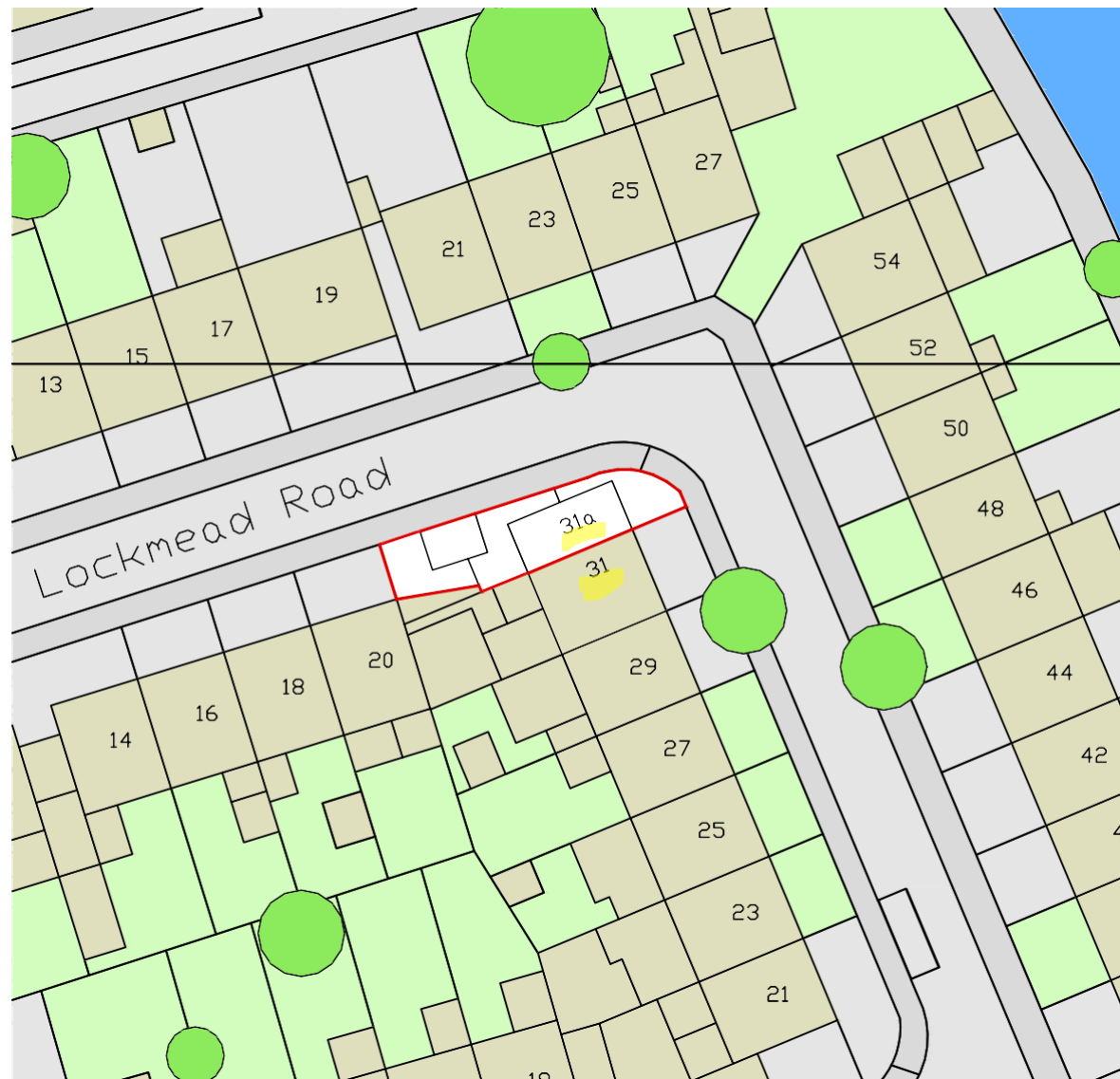
block plan 1:500
