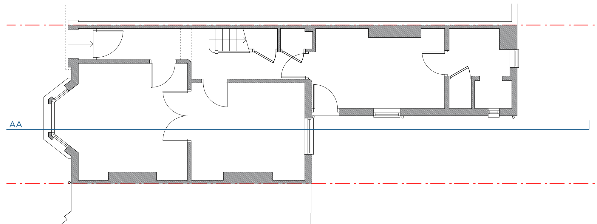
Ground Floor - Existing
