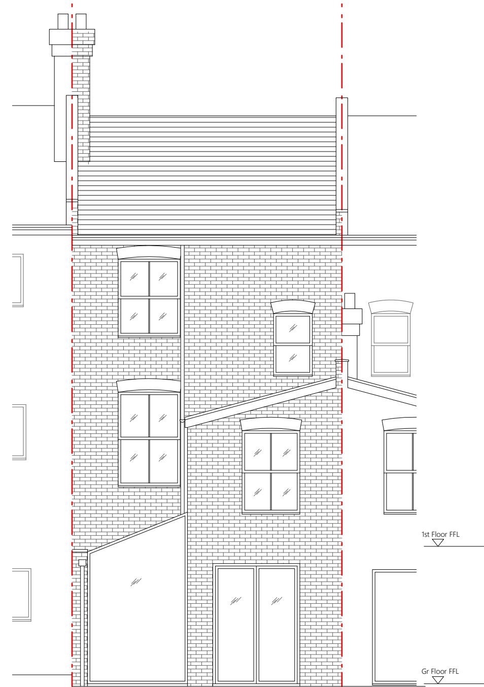
Rear Elevation - Proposal
