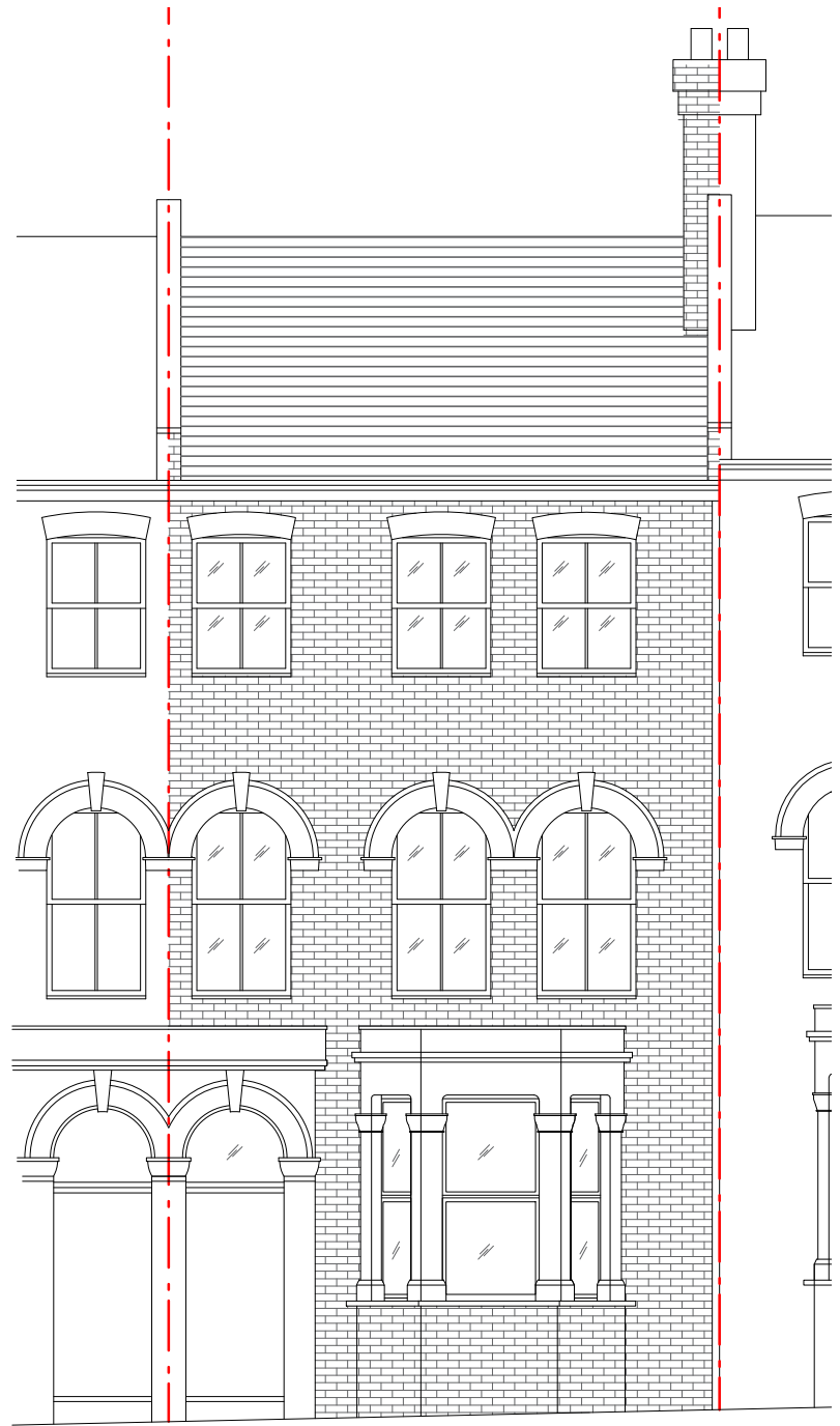
Front Elevation - Proposal
