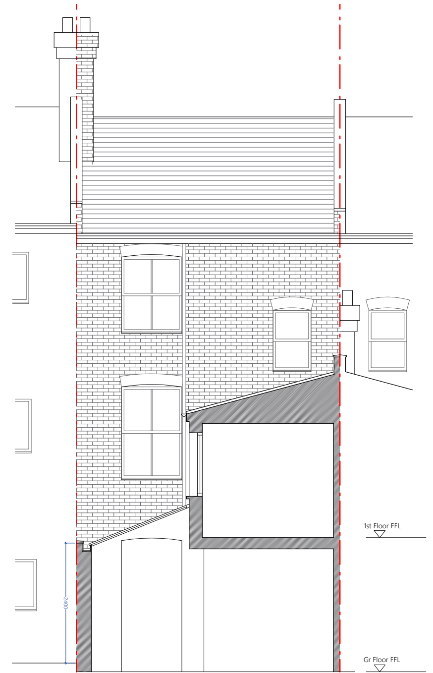
Section BB - Proposal
