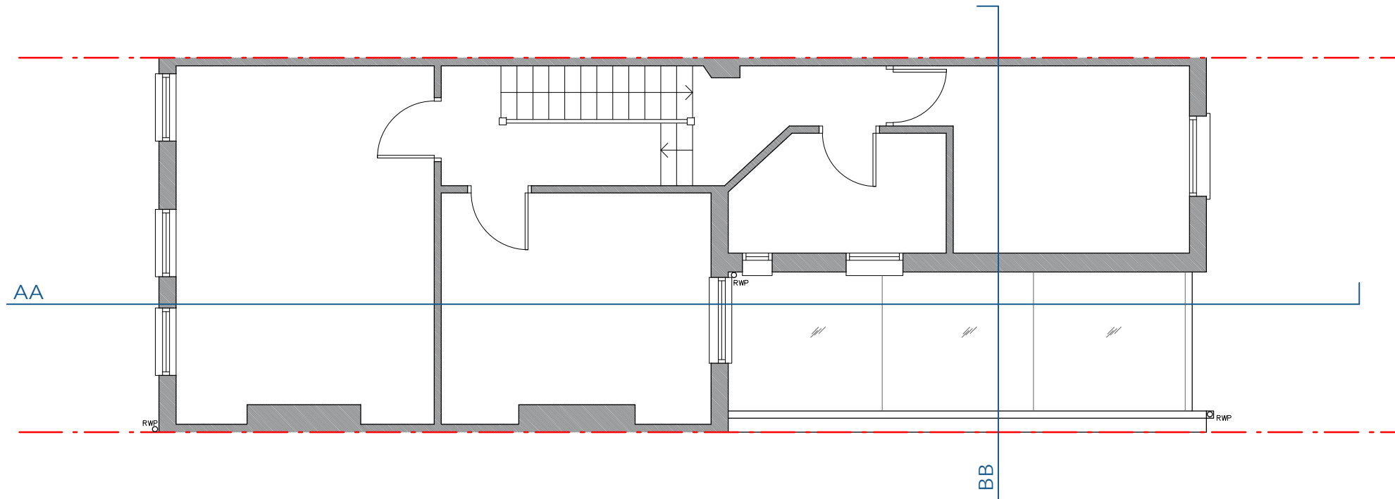
First Floor - Proposed
