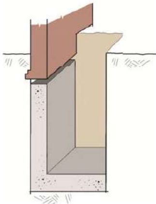
Stage 1. Excavation
