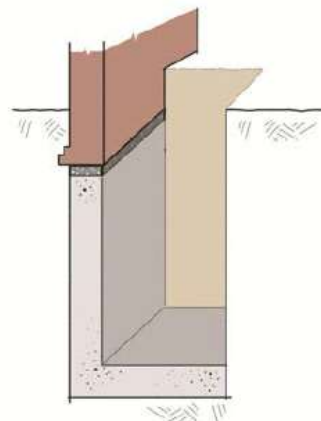
Stage 2. Reinforcement
