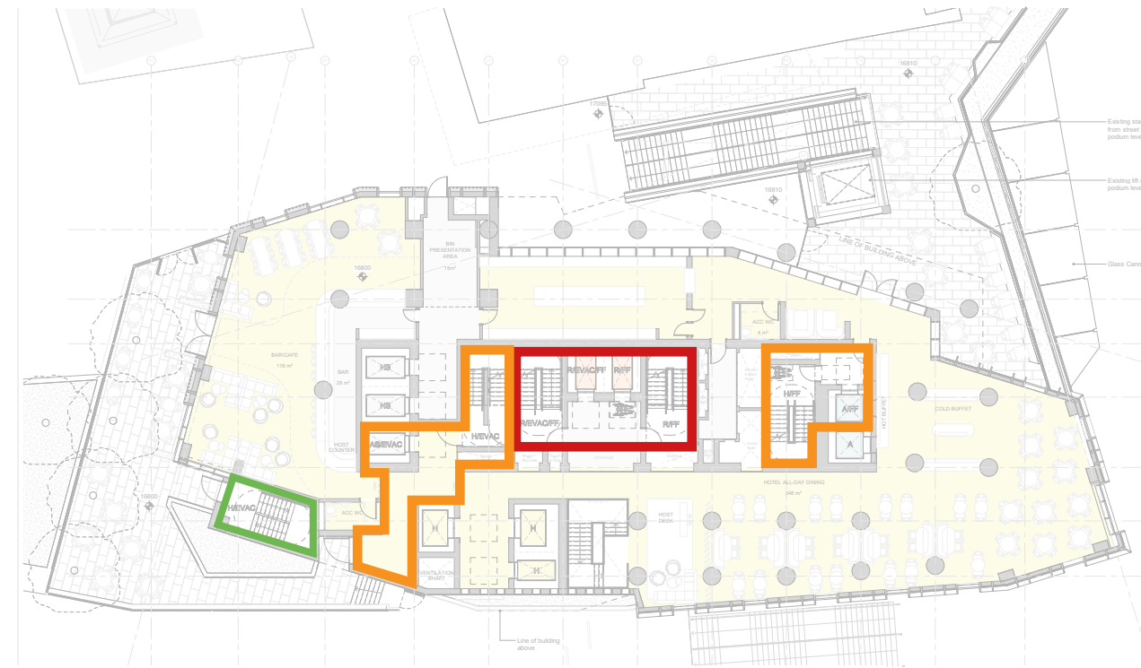
FIGURE 326. Level 01 General Arrangement Plan
