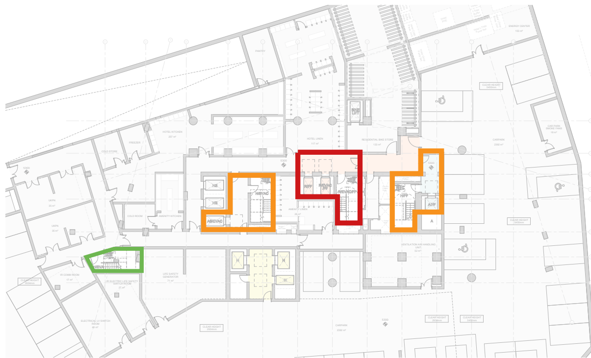
FIGURE 325. Basement General Arrangement Plan
