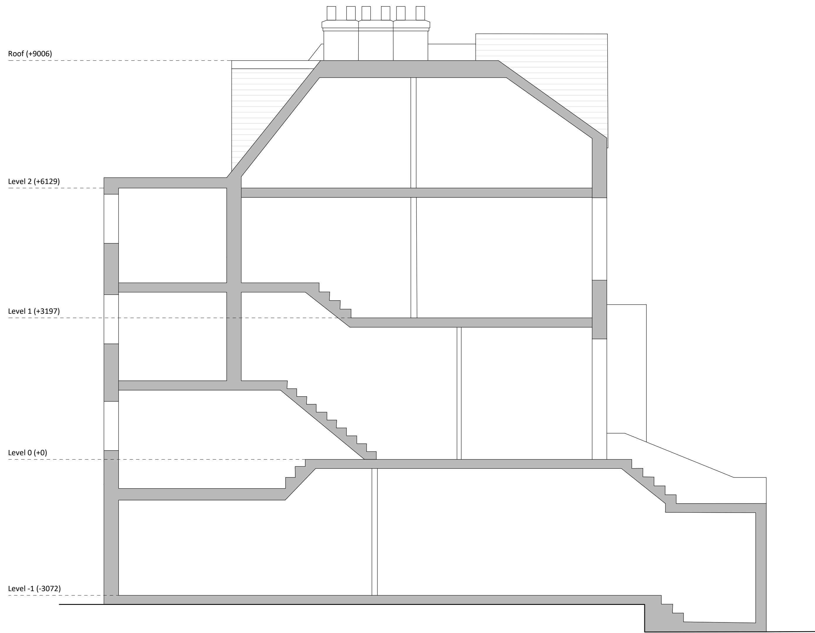
Existing Section
