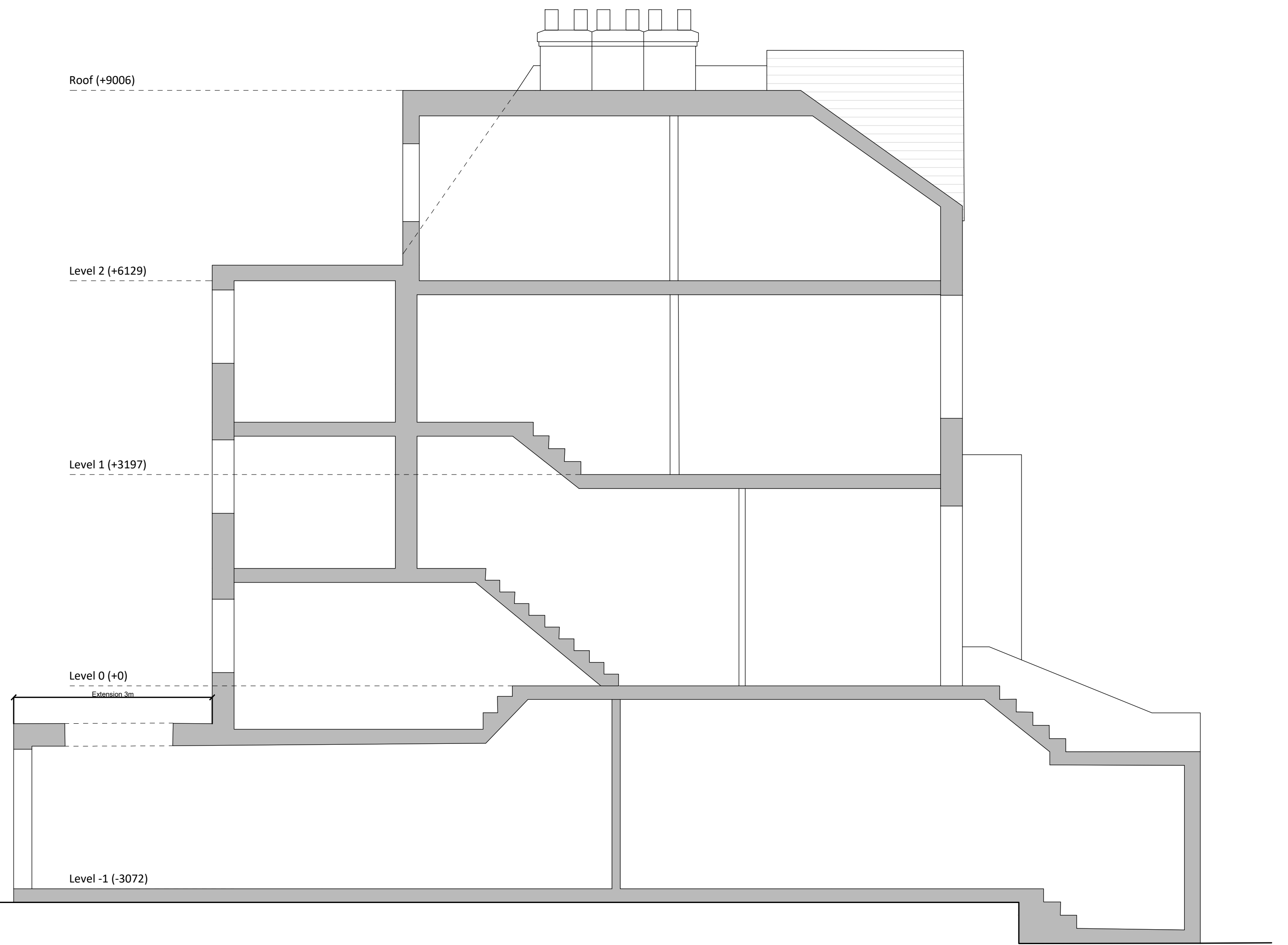
Proposed Section
