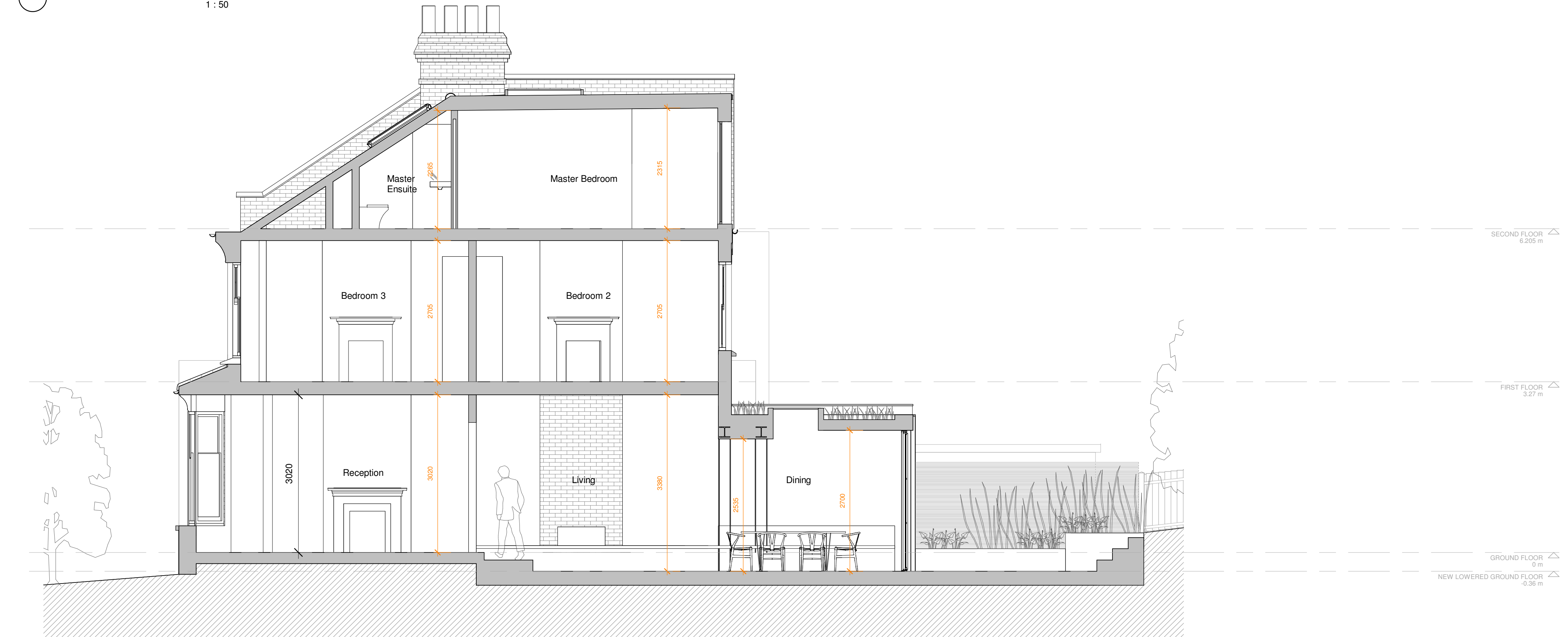
1 Section AA - Proposed 1 : 50
