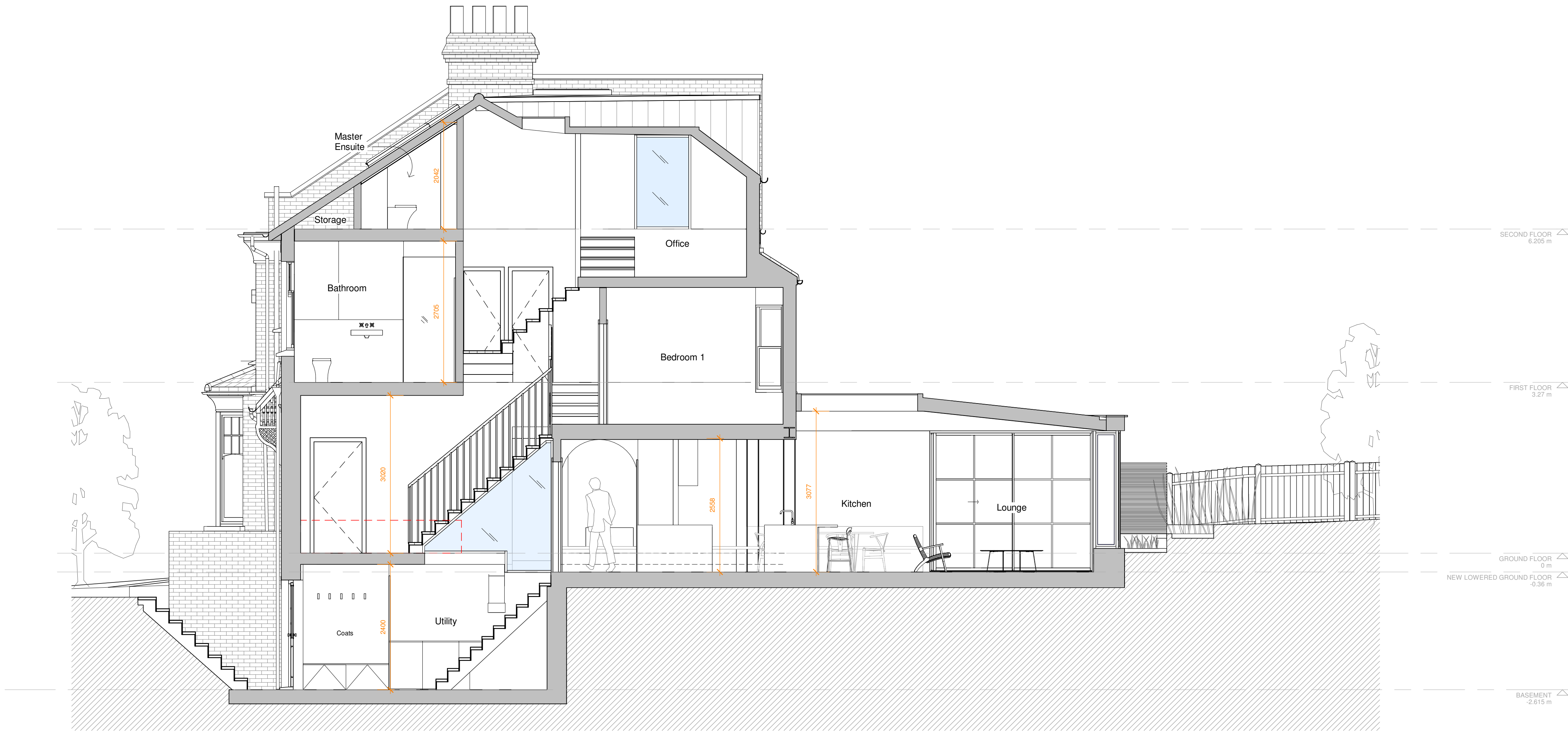
1 Section AA - Proposed 1 : 50
