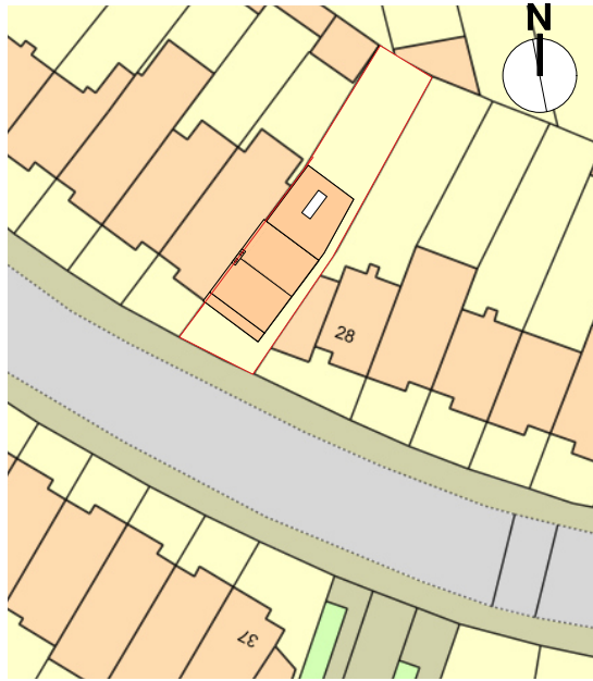
03 PROPOSED BLOCK PLAN Scale: 1:500
