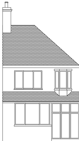
04 EXISTING FRONT ELEVATION Scale: 1:50
