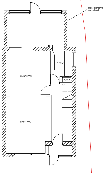
01 EXISTING GROUND FLOOR Scale: 1:50
