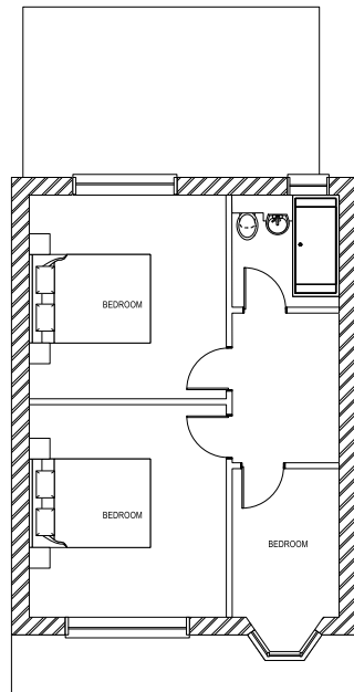
02 EXISTING 1ST FLOOR Scale: 1:50
