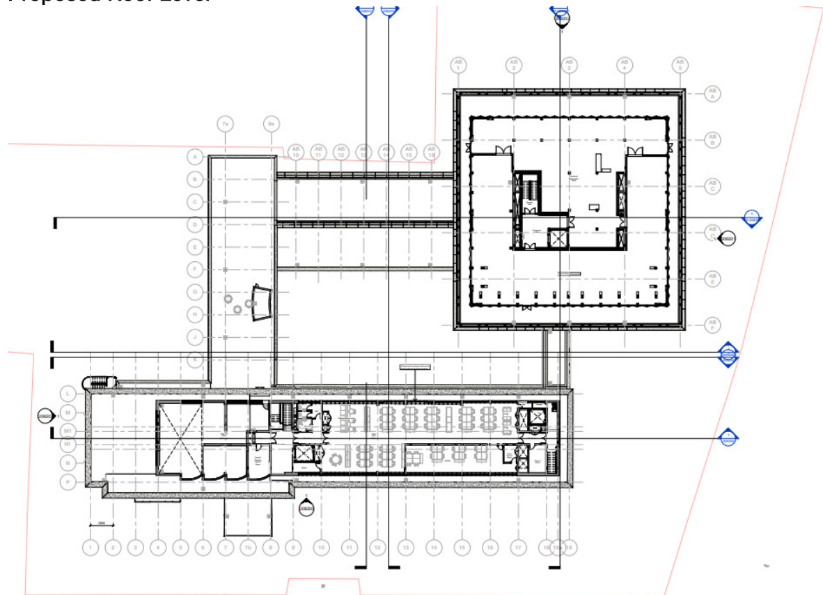
Proposed Roof Level
