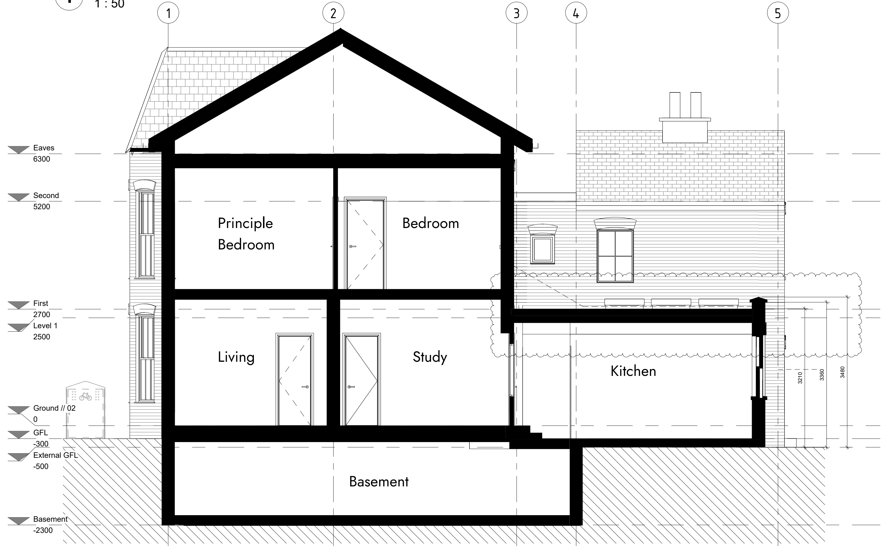
2 Proposed // Section 2 1 : 50
