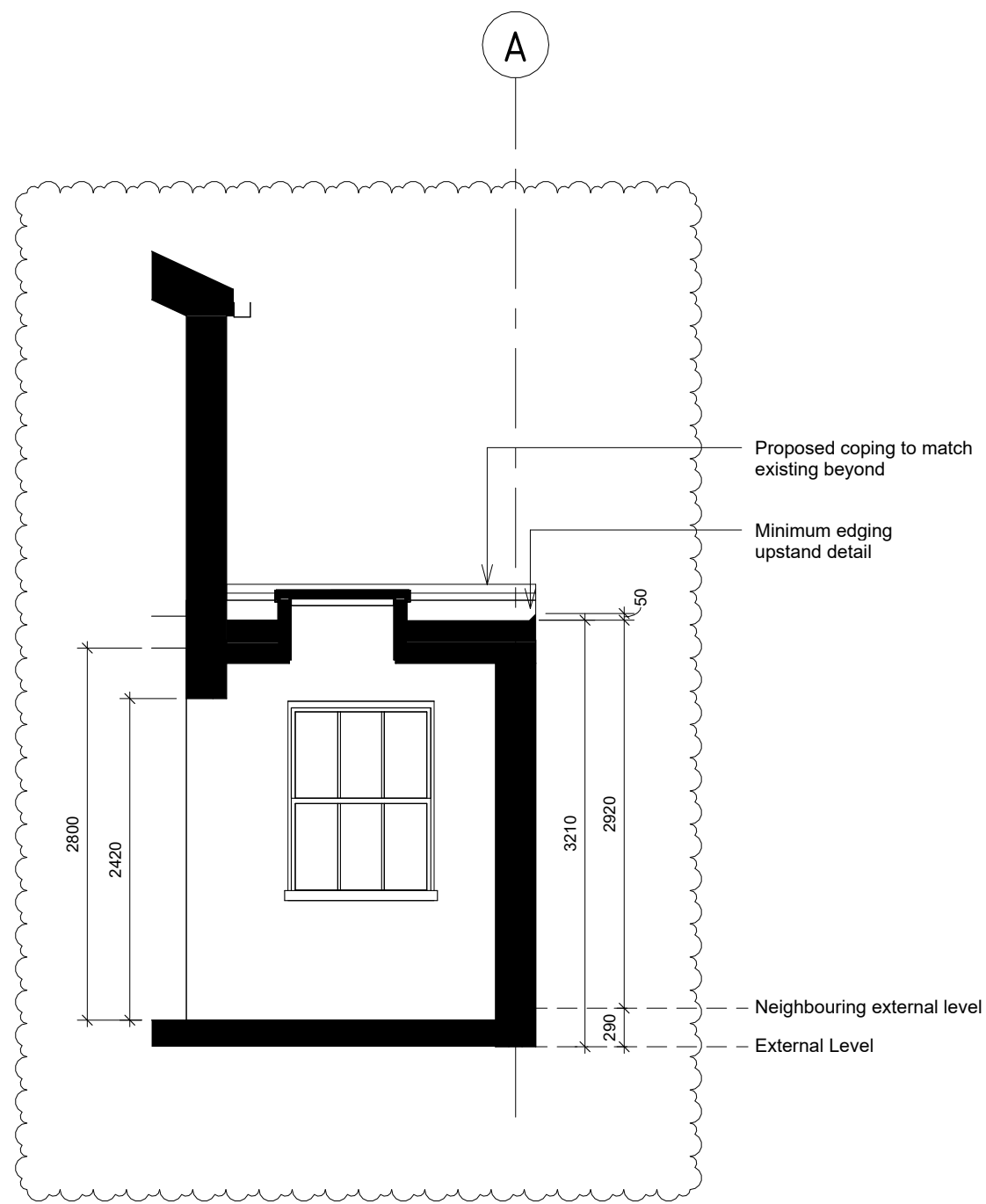
3 Proposed // Section 3 1 : 50
