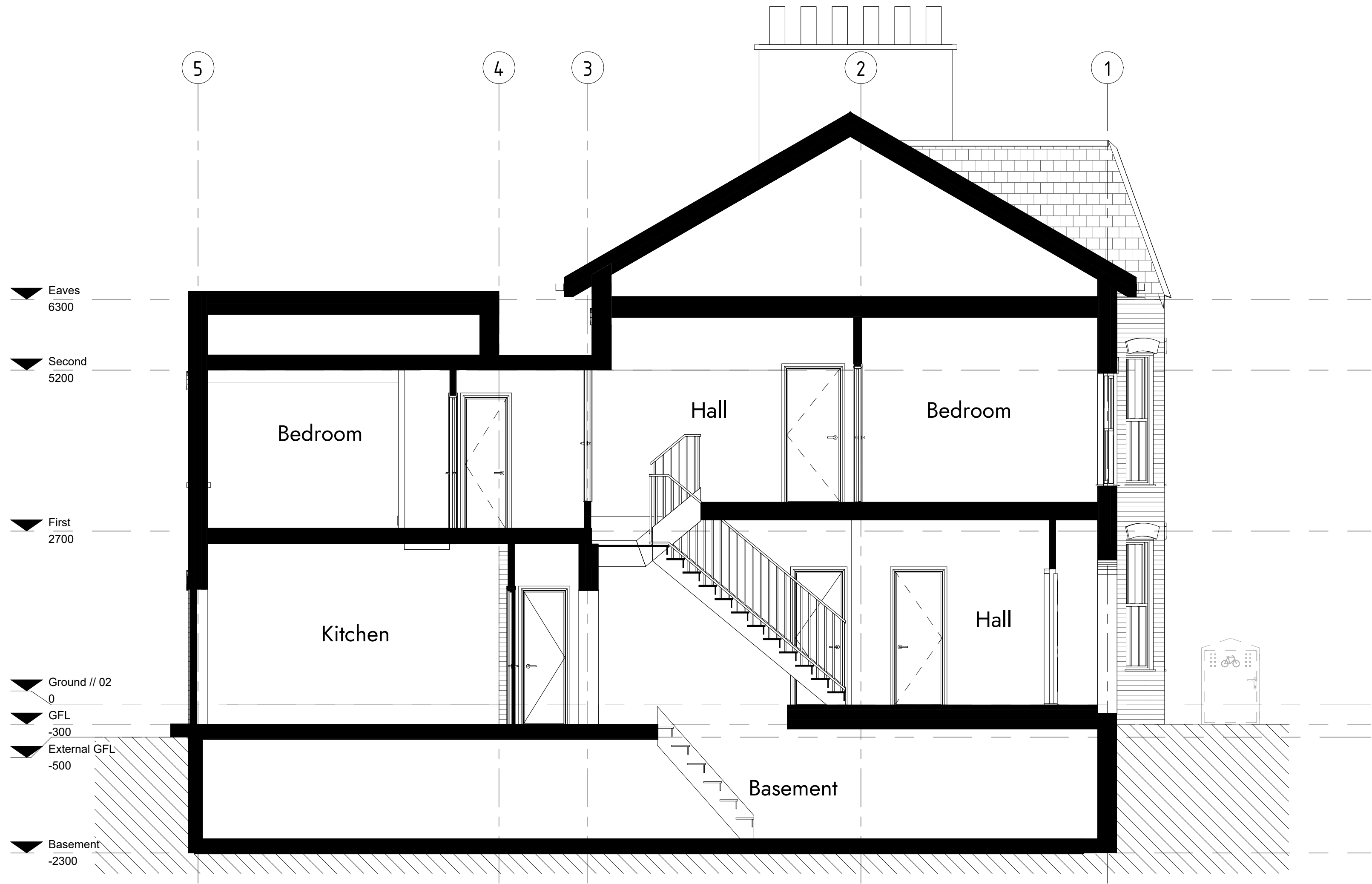
1 Proposed // Section 1 1 : 50
