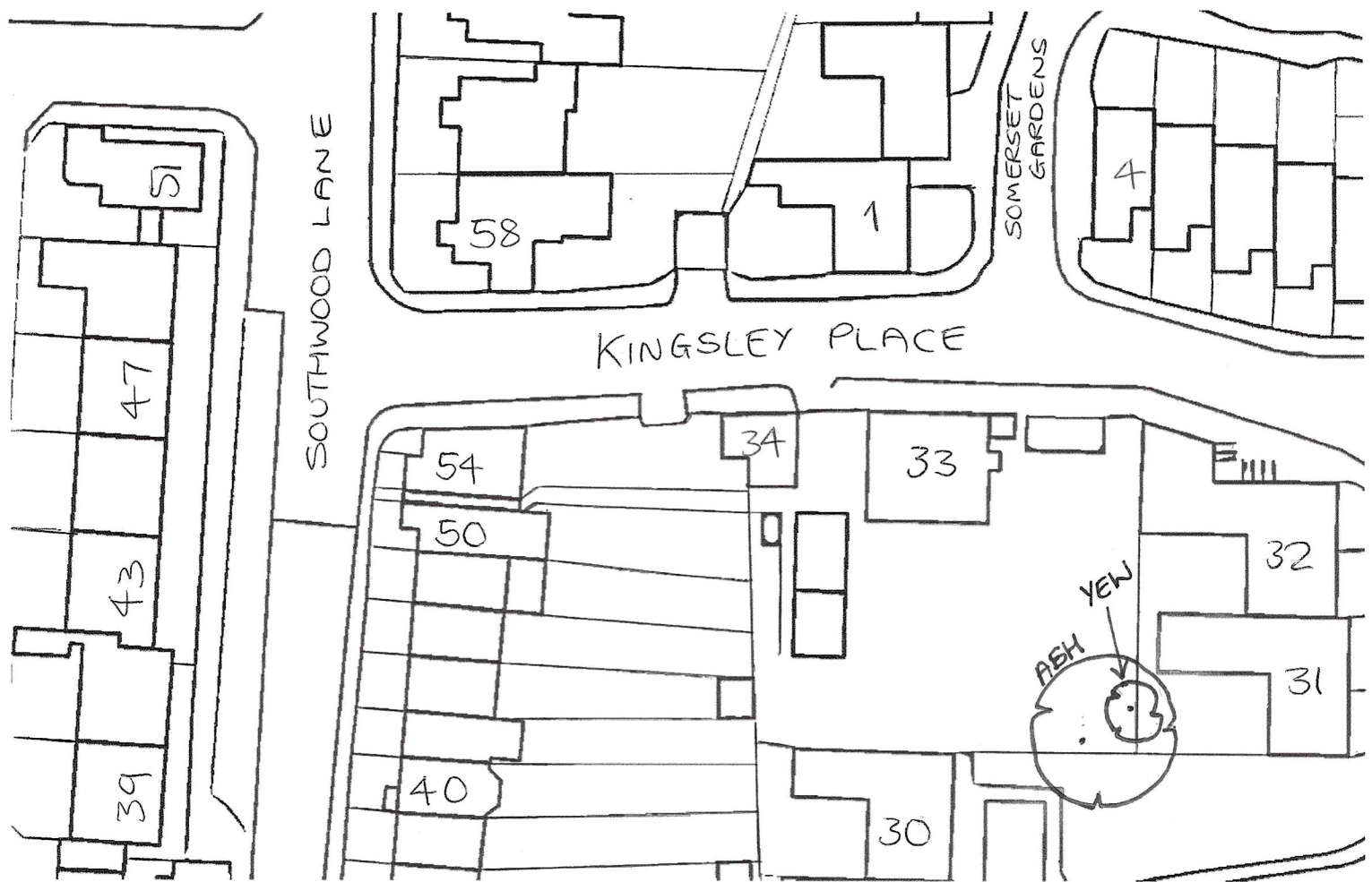
SITE PLAN FOR 33, KINGSLEY PLACE, LONDON, N6 SEA
