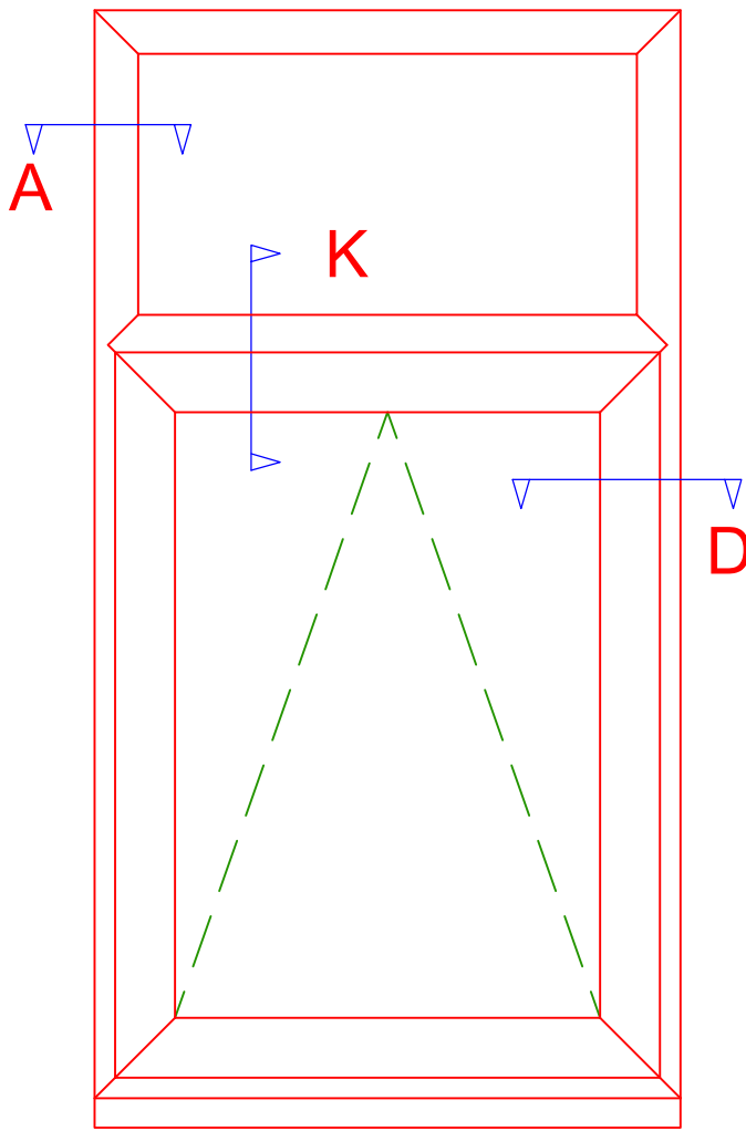
PROPOSED WINDOW TYPE - W1, W2
