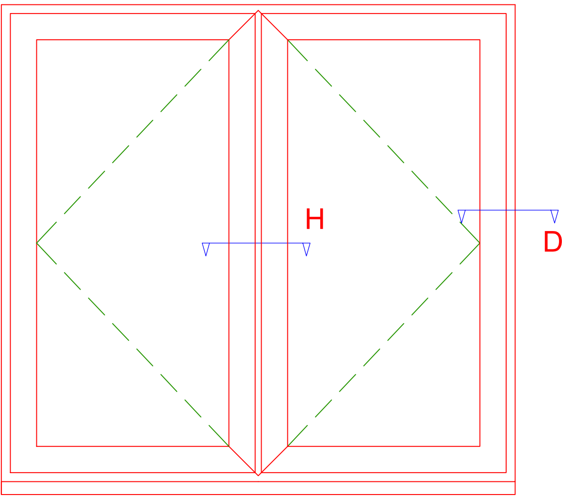
PROPOSED WINDOW TYPE - W8
