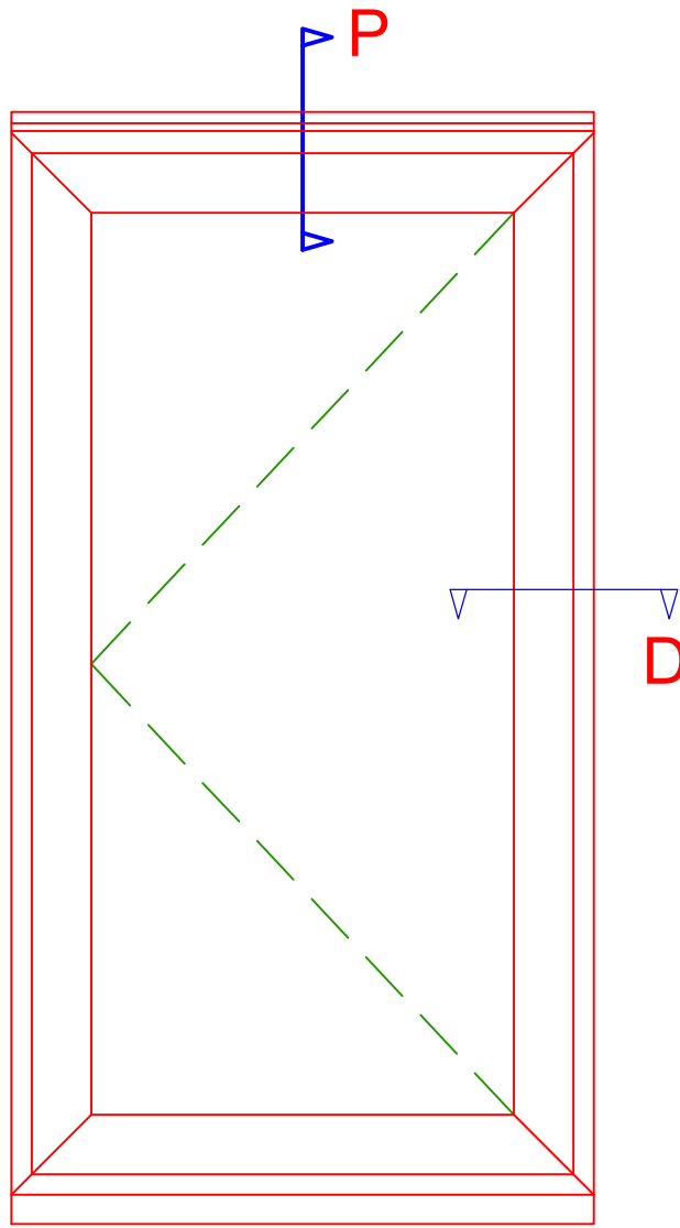
PROPOSED WINDOW TYPE - W9
