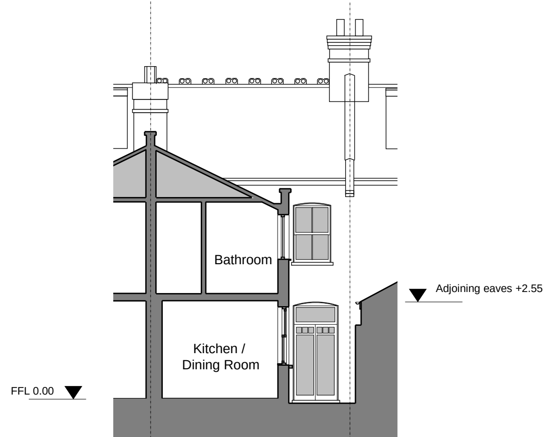
Section C-C
