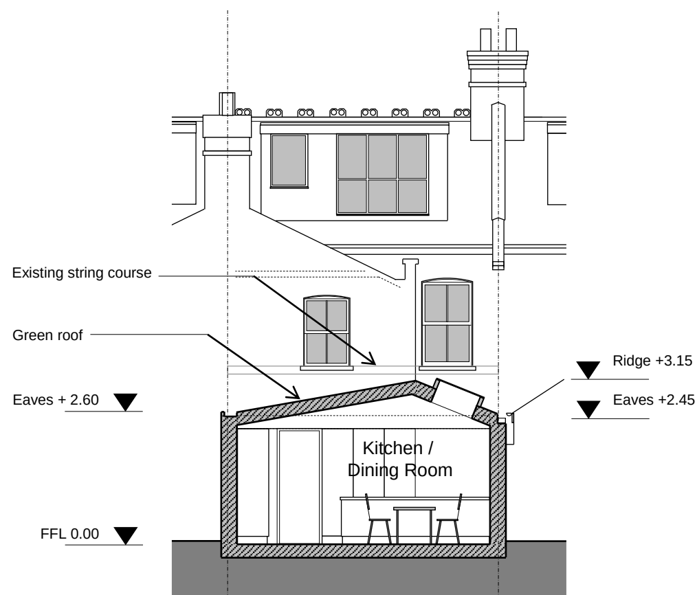
Section E-E
