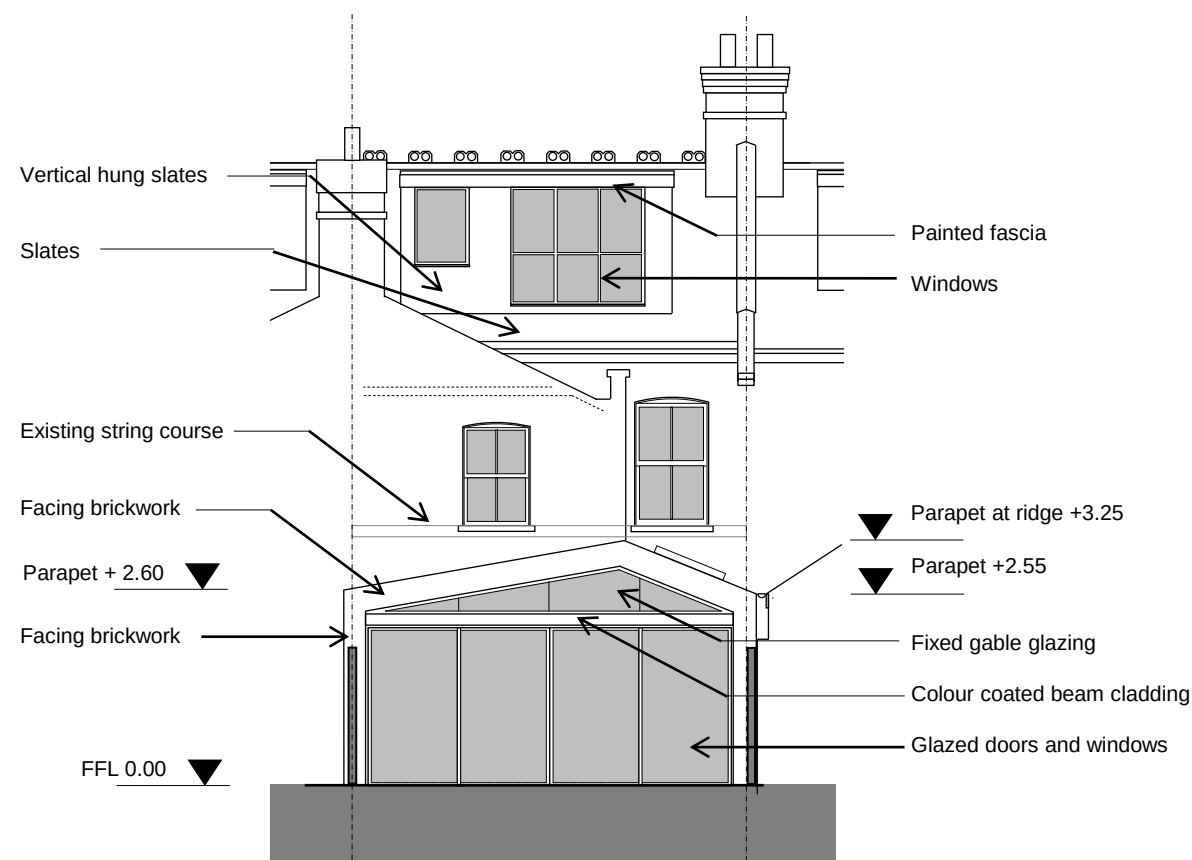
Rear Elevation – Section D-D
