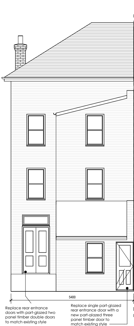
PROPOSED REAR ELEVATION 1 : 50
