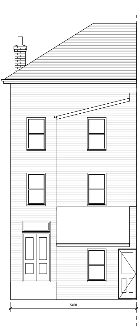
EXISTING REAR ELEVATION 1 : 50
