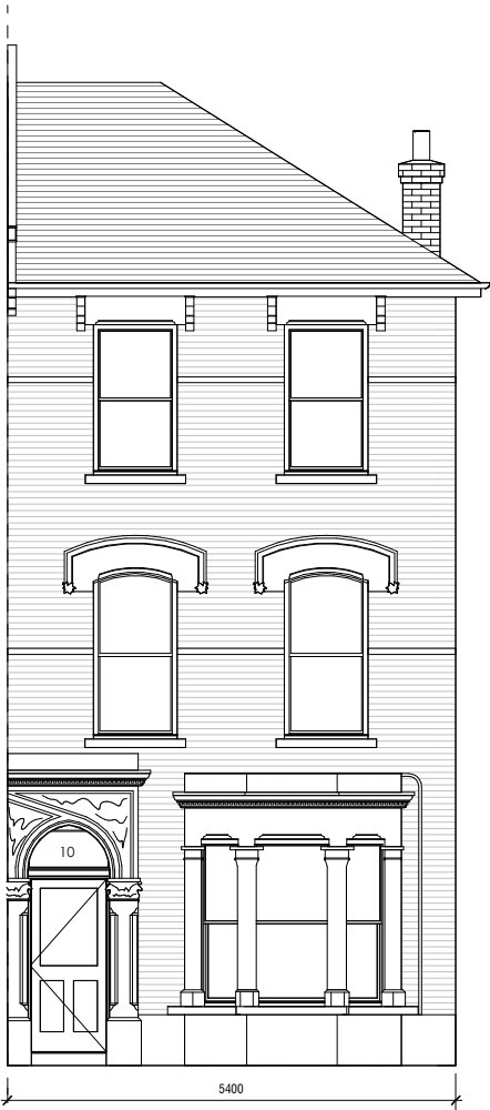
PROPOSED FRONT ELEVATION 1 : 50
