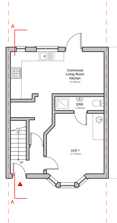
PROPOSED GROUND FLOOR
