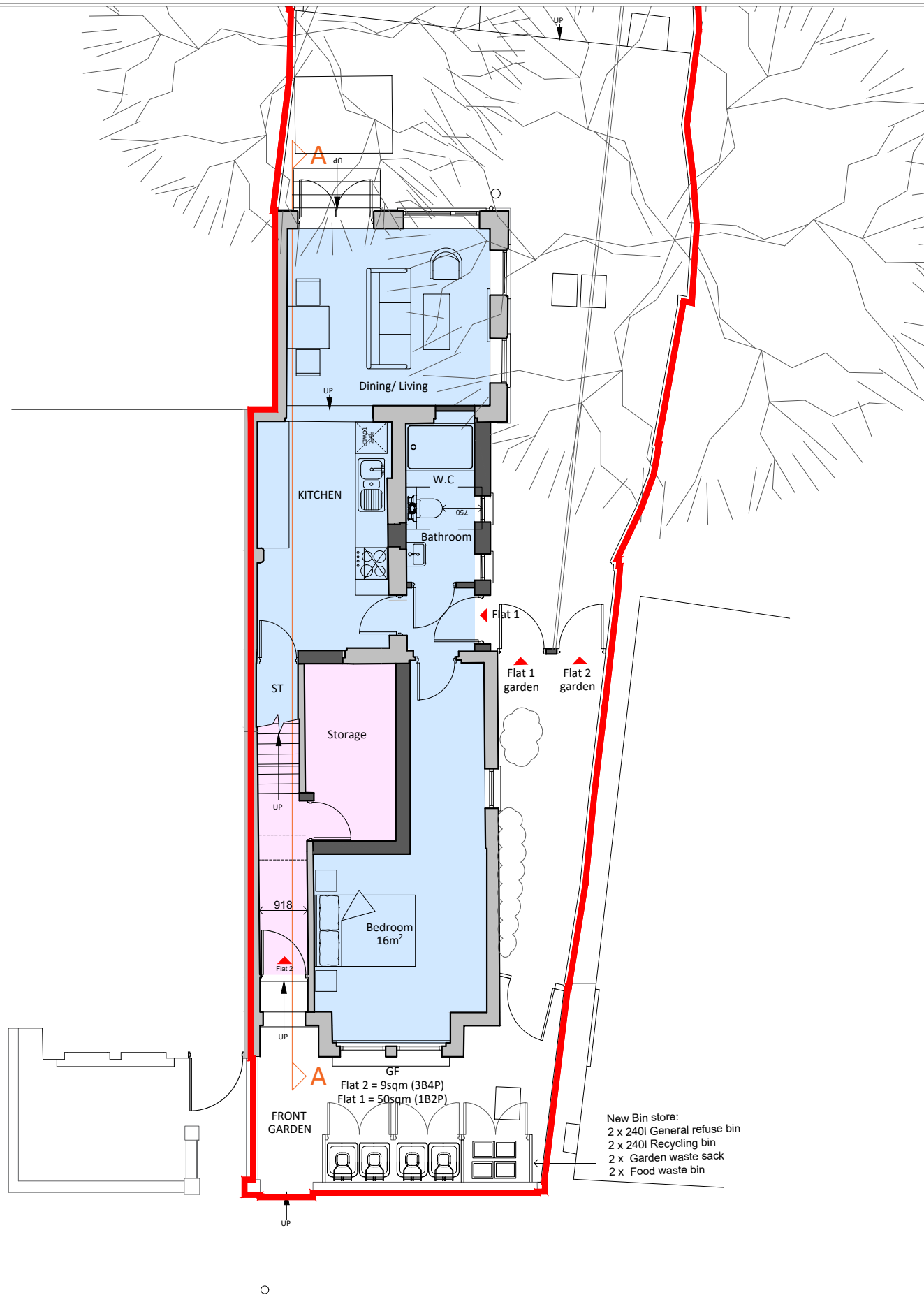
Proposed G Floor Plan
