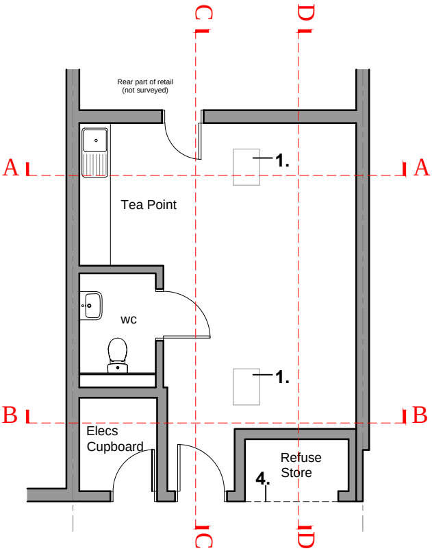
FLOOR PLAN - AS PROPOSED
