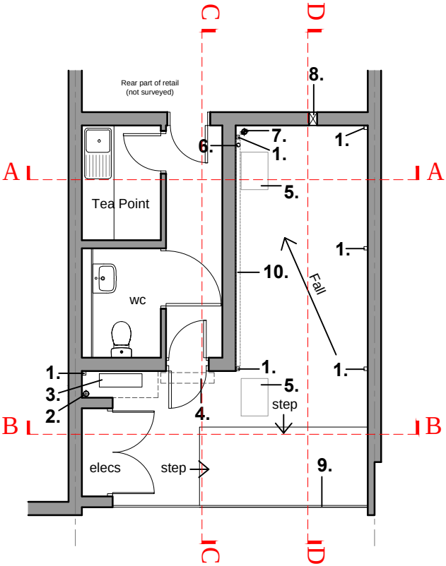
FLOOR PLAN - AS EXISTING
