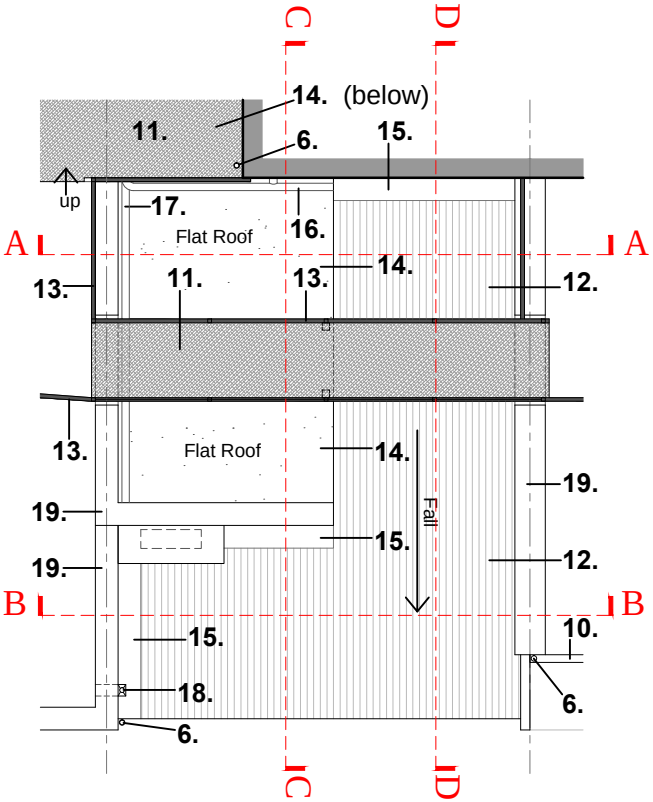
ROOF PLAN - AS EXISTING
