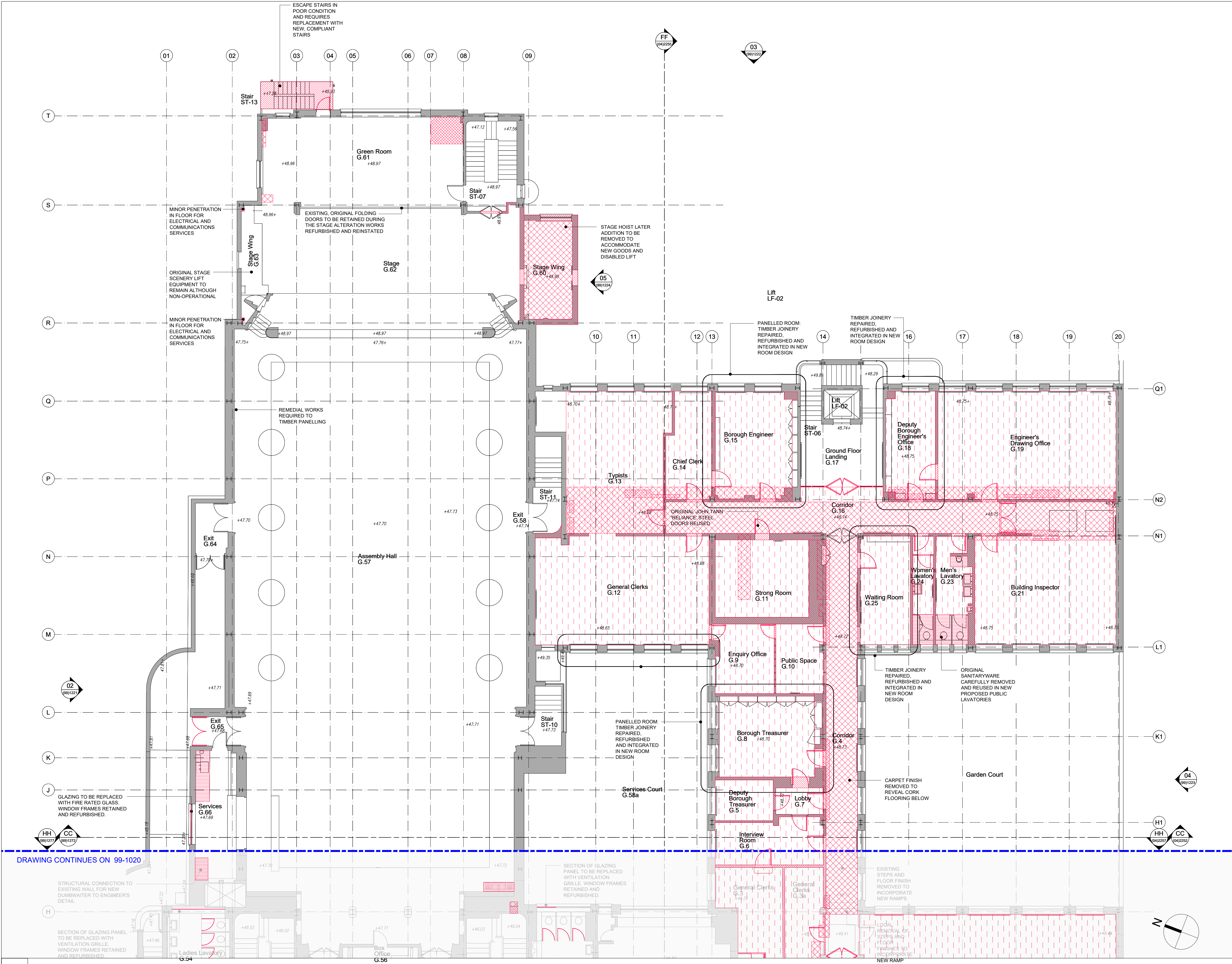
DEMOLITION PLAN - GROUND FLOOR EAST
