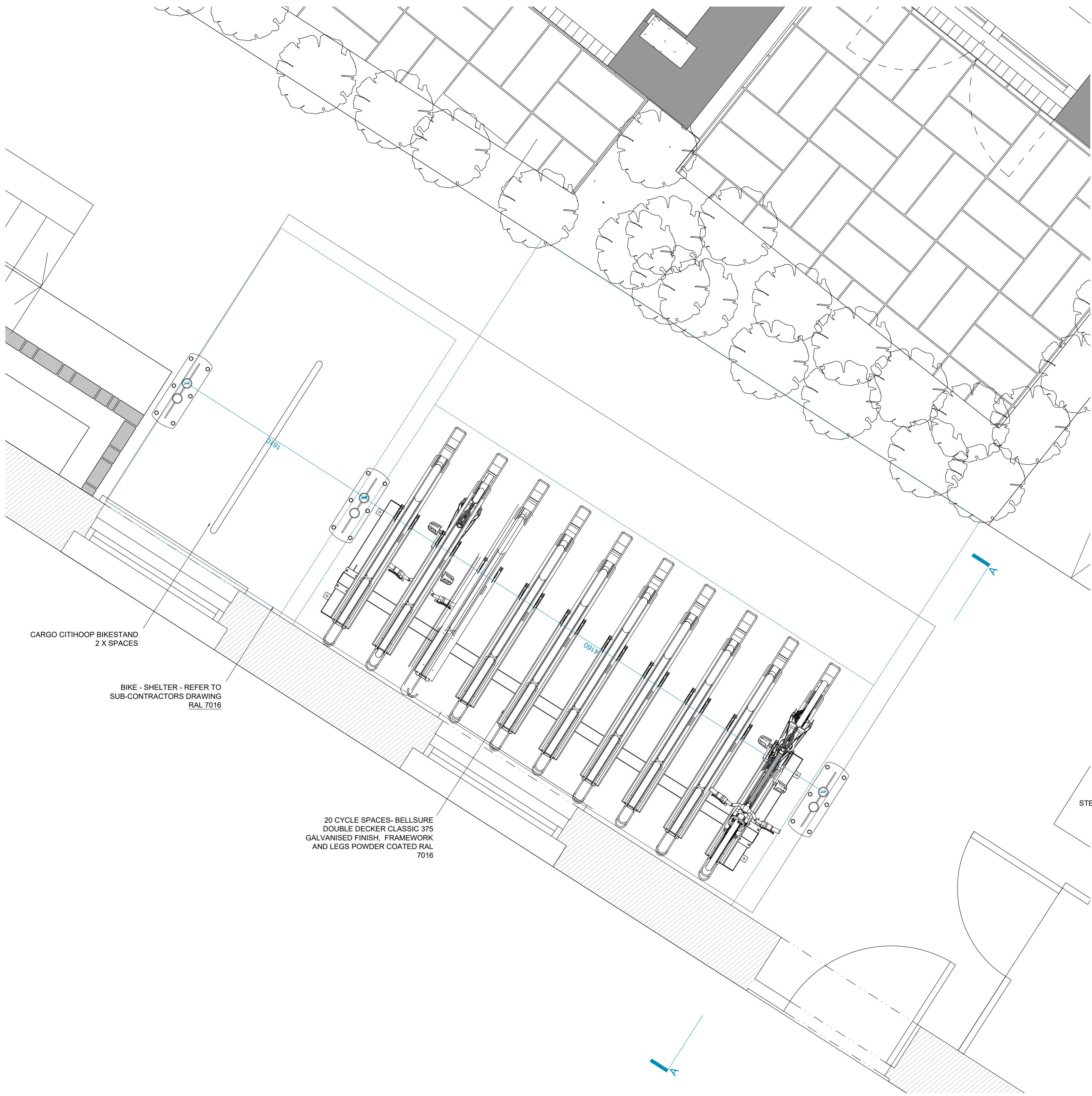
CYCLE STORE PLAN
