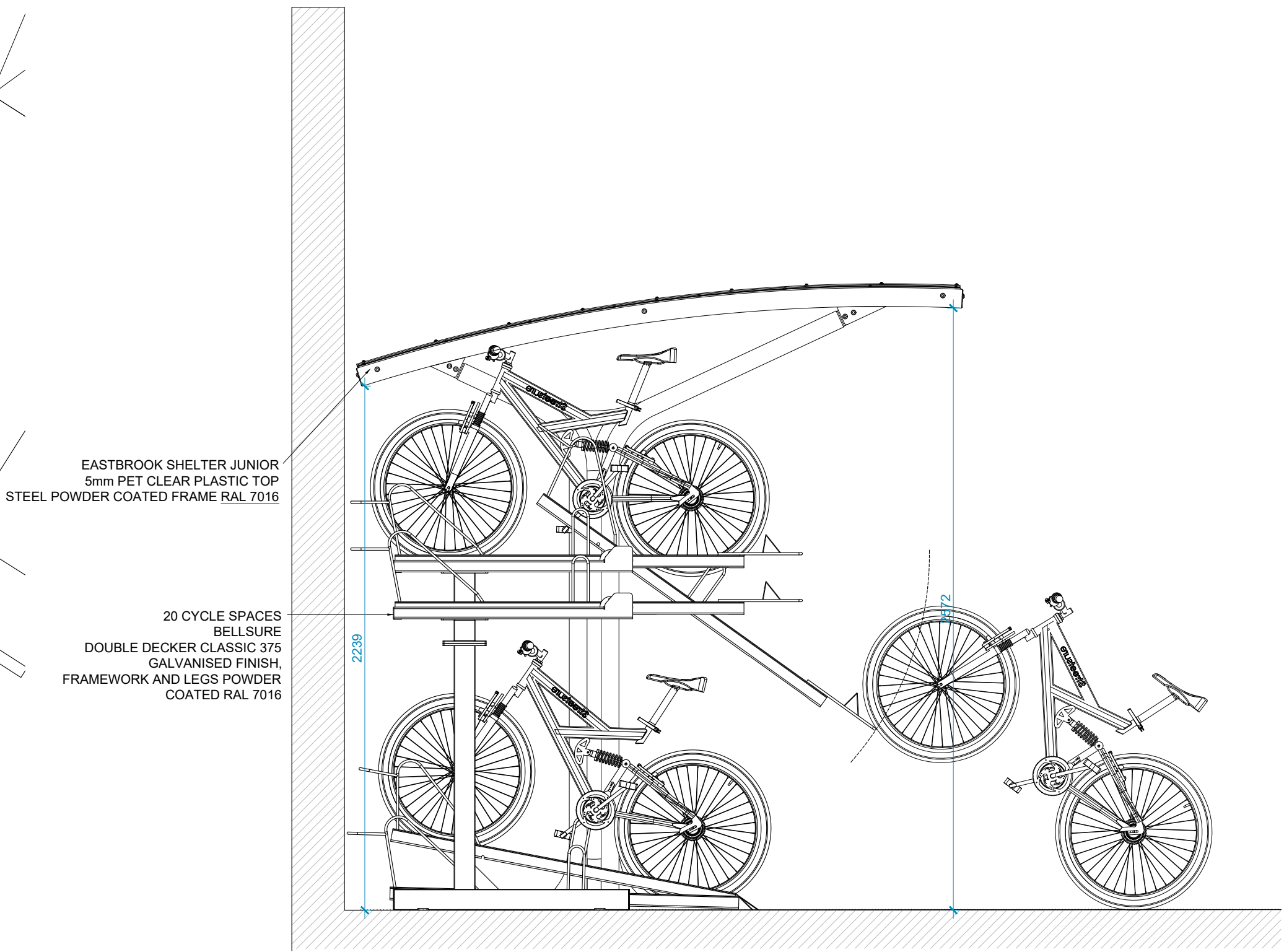
CYCLE STORE VIEW A-A
