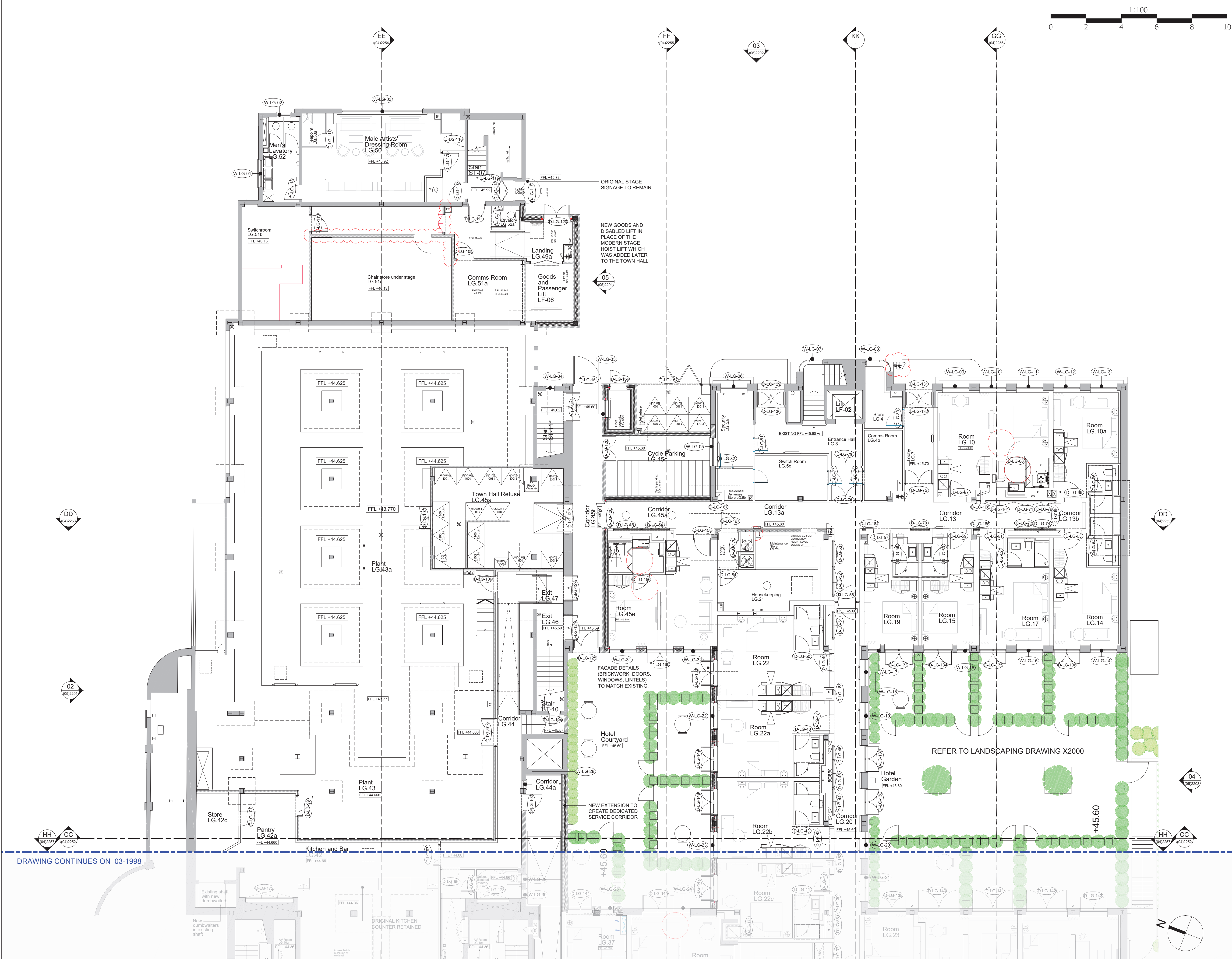
- PROPOSED PLAN - LOWER GROUND FLOOR EAST
