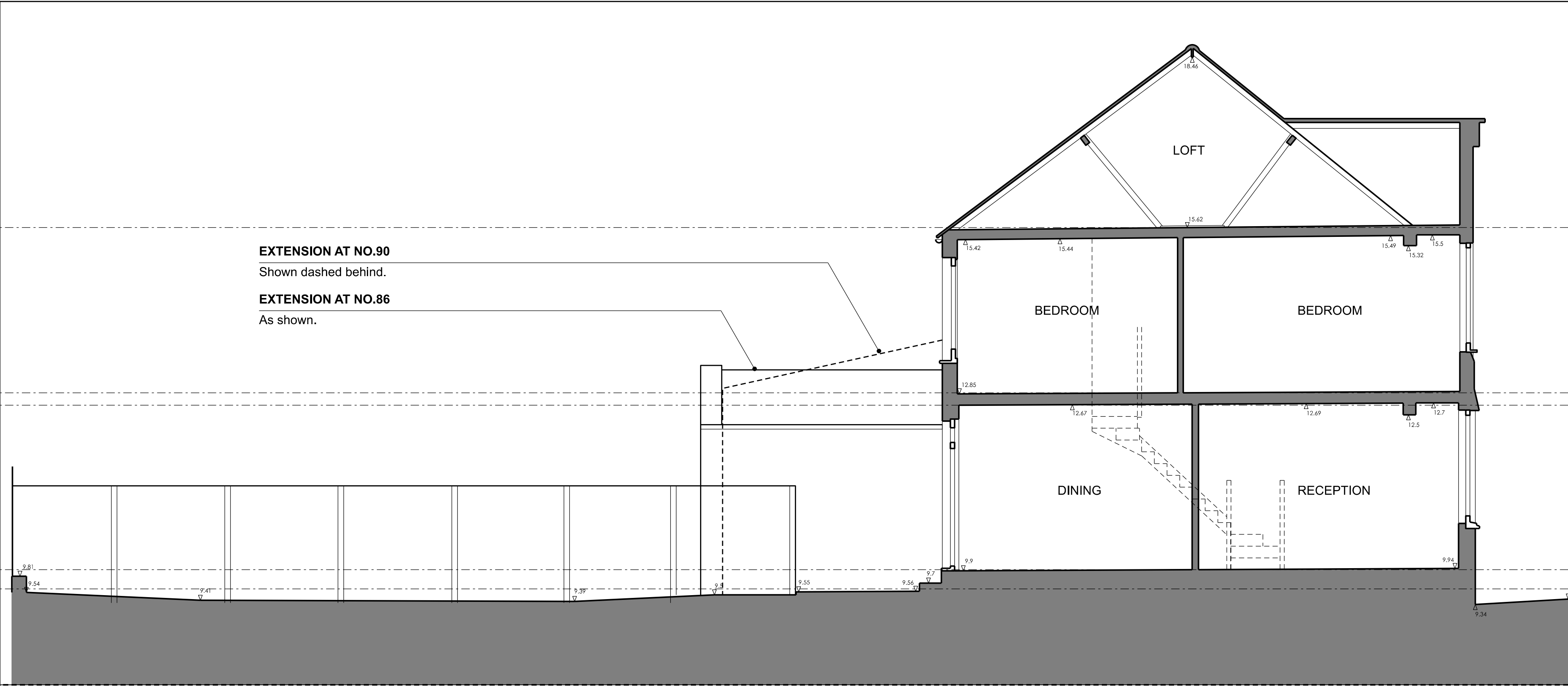
01 EXISTING LONG SECTION SCALE 1:100 @A3
