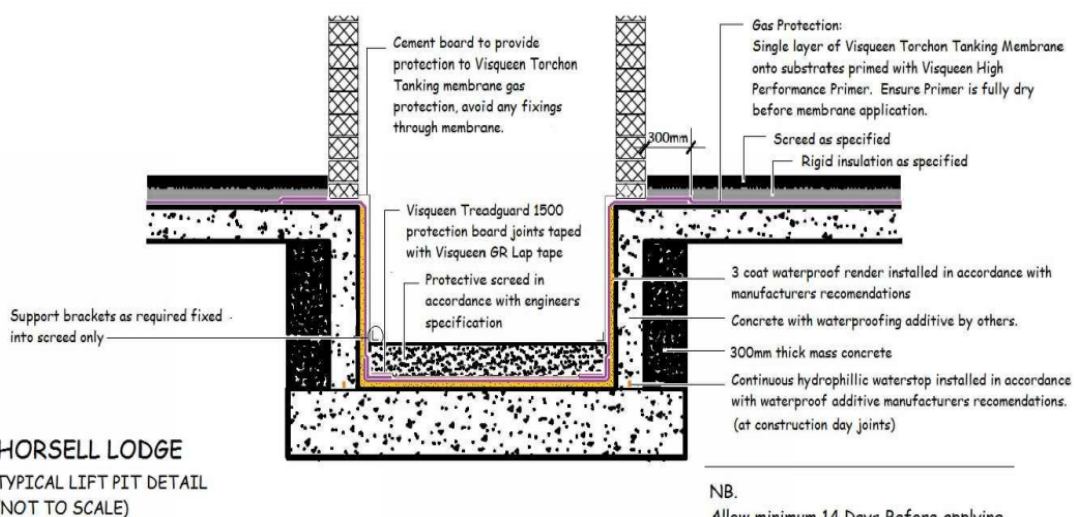
TYPICAL RETAINING WALL DETAIL AT LIGHTWELL SCALE 1:20
