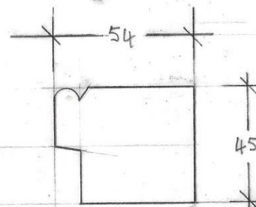
Casement window centre stile section "French Meeting" (1:2 scale)
