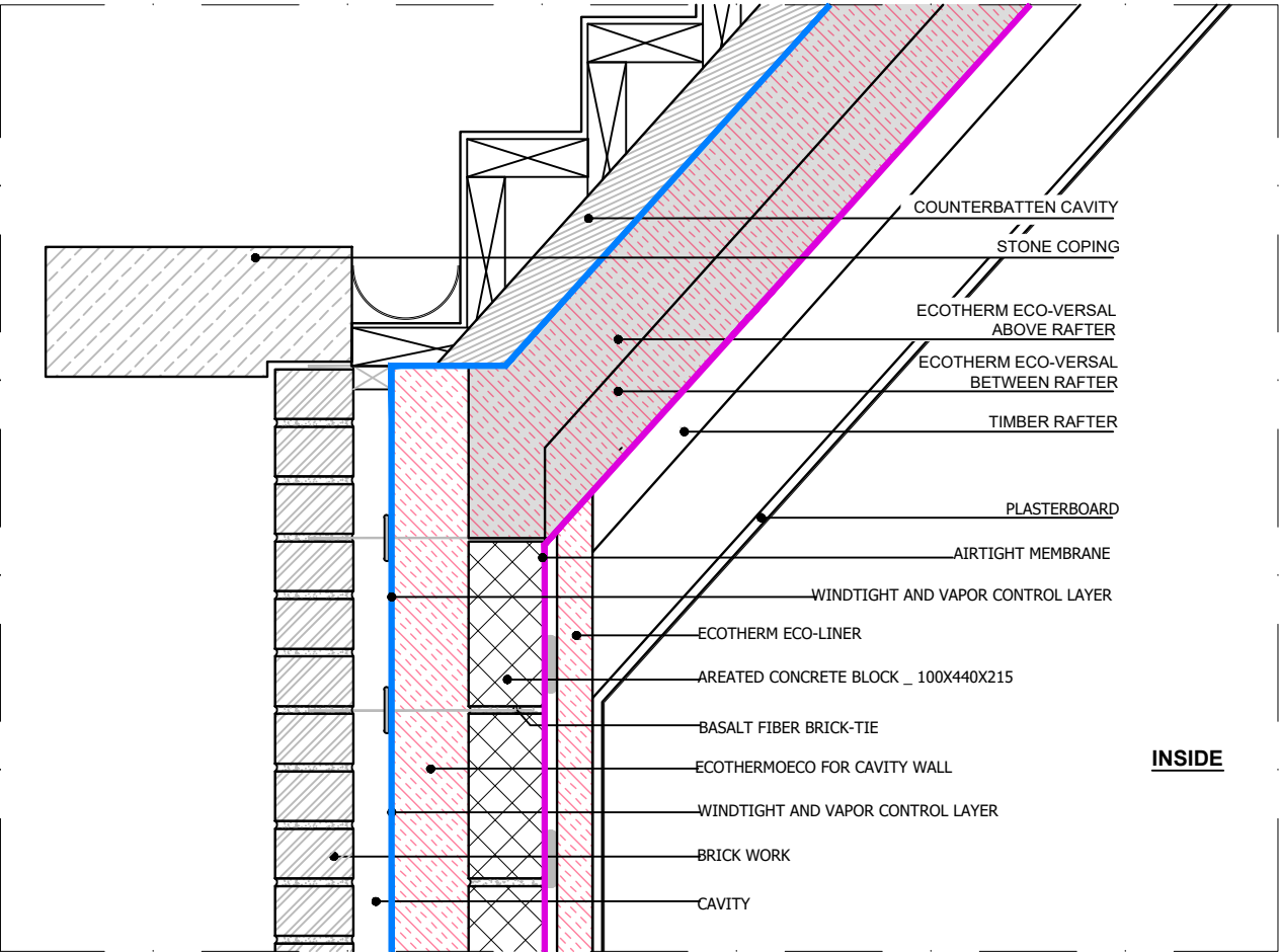
WALL TYPE 1 / PITCHED ROOF _ SECTION DETAIL
