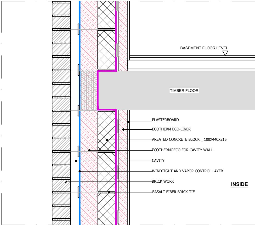
WALL TYPE 1 / INTERMEDIATE FLOOR _ SECTION DETAIL
