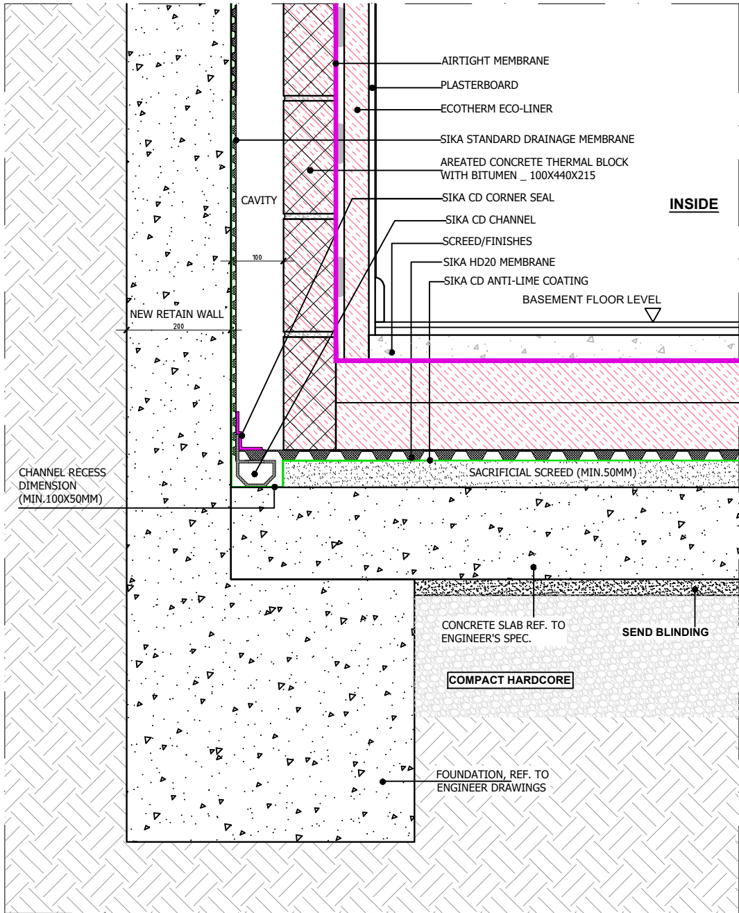
WALL TYPE 4 / BASEMENT FLOOR _ SECTION DETAIL
