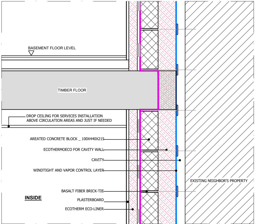
WALL TYPE 2 / TO NEIGHBOR'S _ SECTION DETAIL
