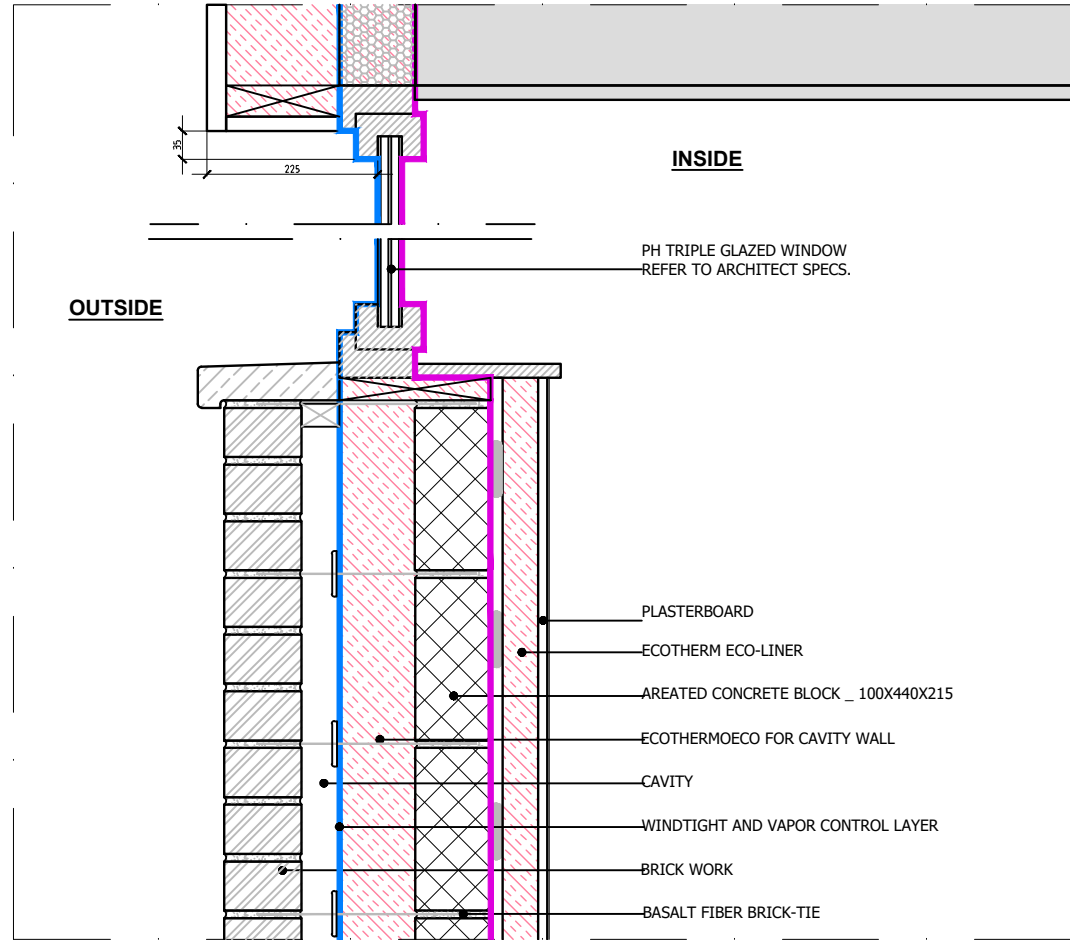
WALL TYPE 1 / WINDOW _ SECTION DETAIL
