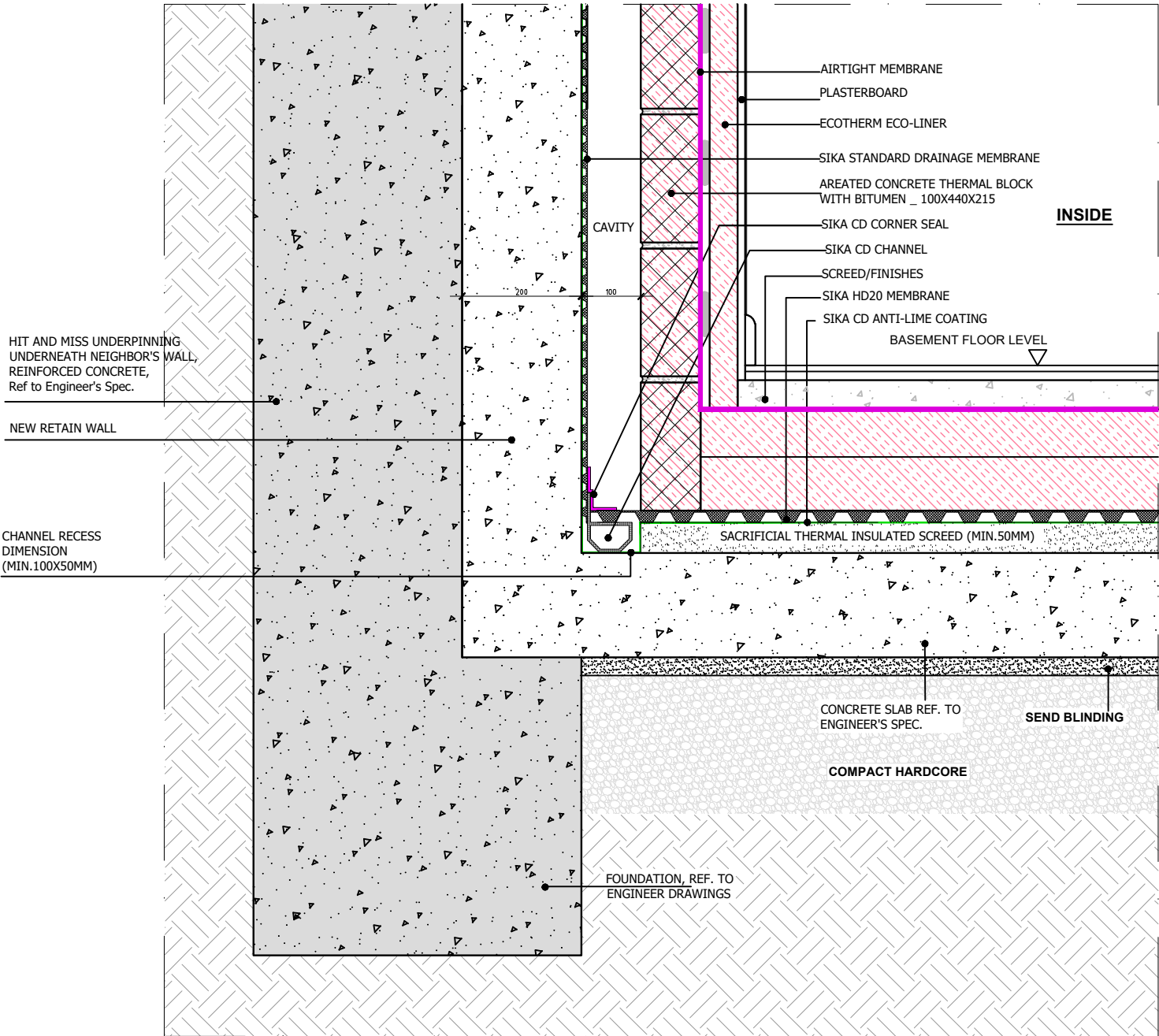
WALL TYPE 3 / BASEMENT FLOOR _ SECTION DETAIL
