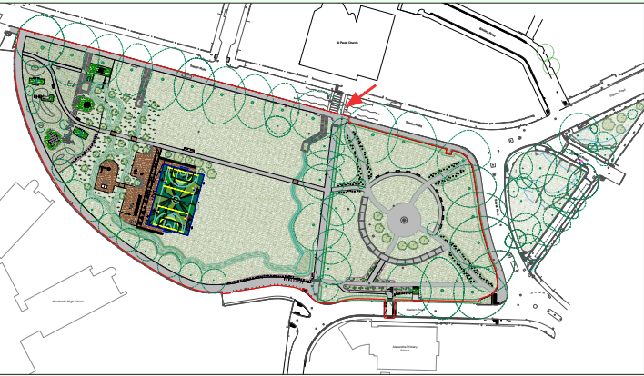
Proposed Plan
